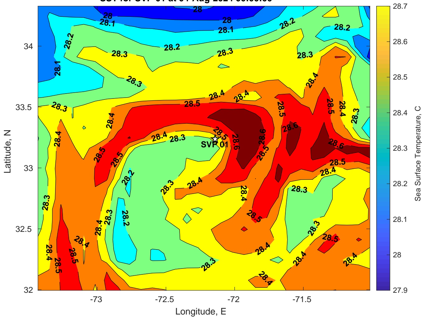
SST for SVP 01 at 04-Aug-2024 00:00:00
