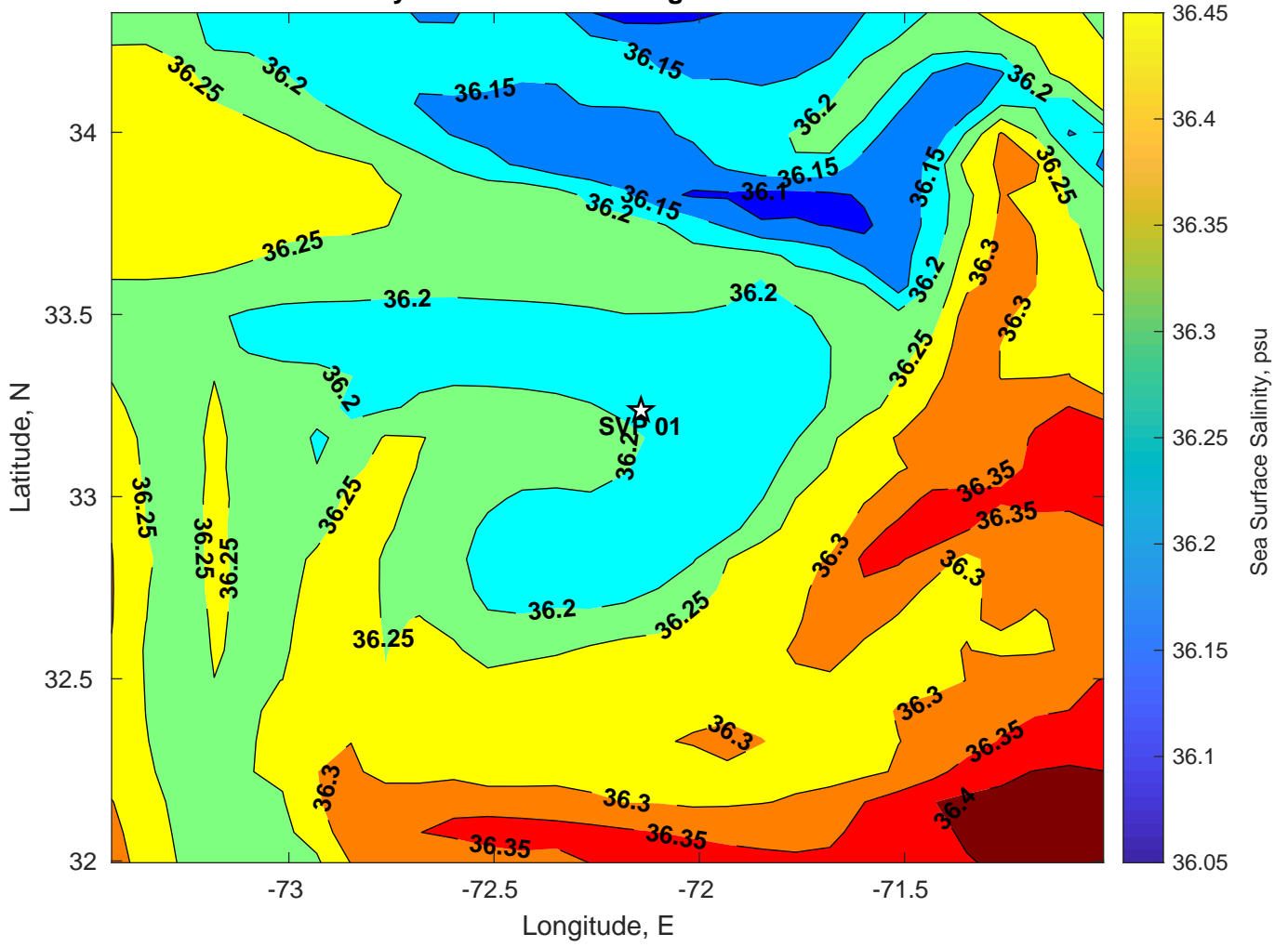
Surface Salinity for SVP 01 at 04-Aug-2024 00:00:00
