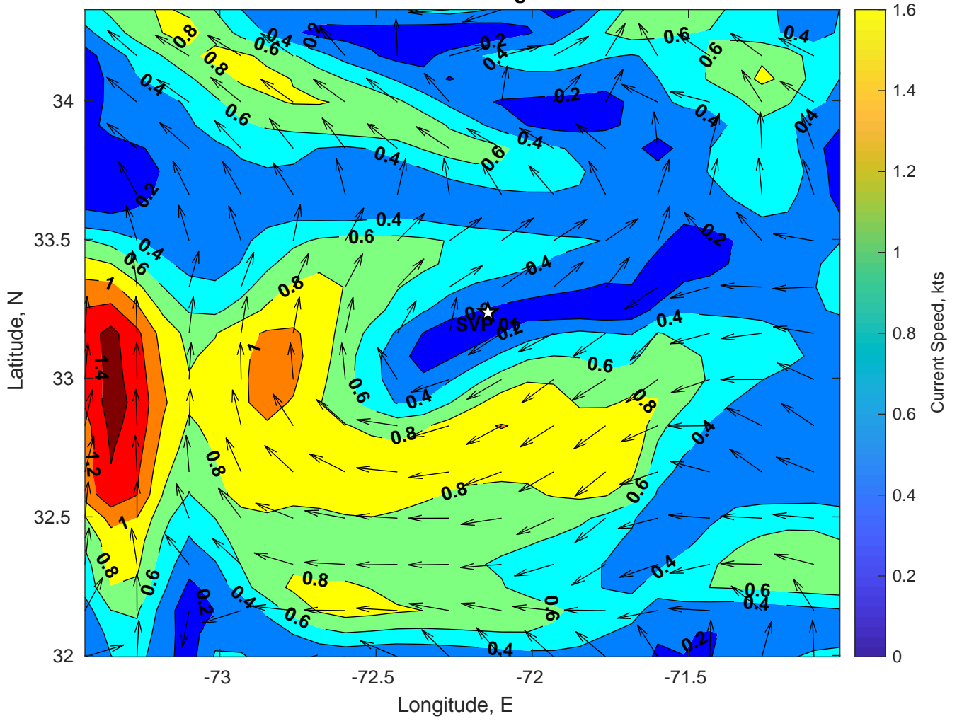
Surface Currents for SVP 01 at 04-Aug-2024 00:00:00
