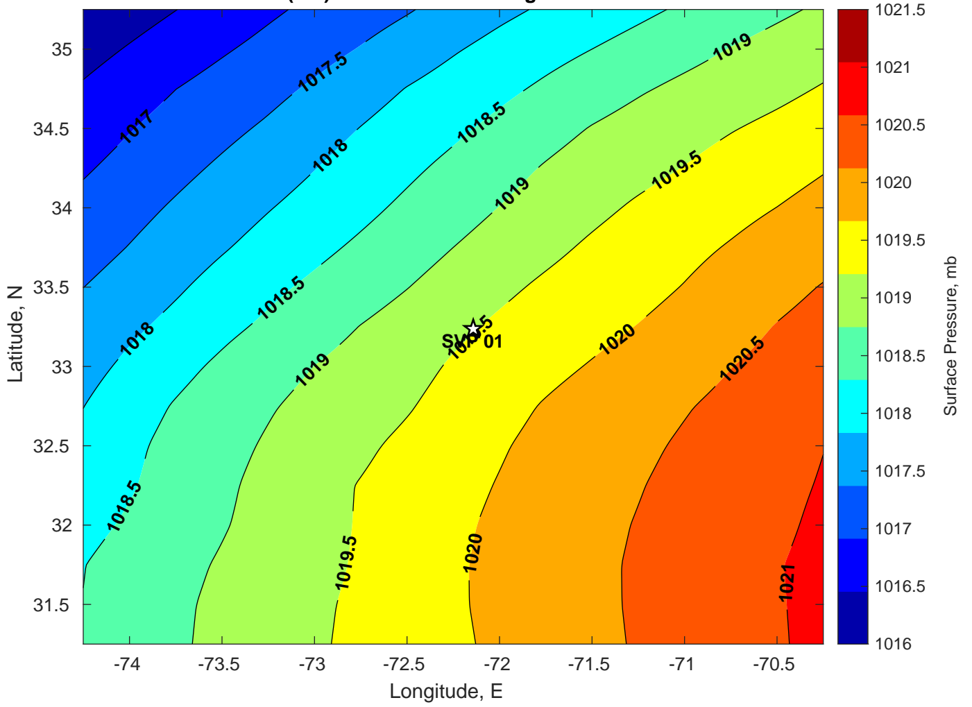
Surface Pressure (mb) for SVP 01 at 04-Aug-2024 00:00:00
