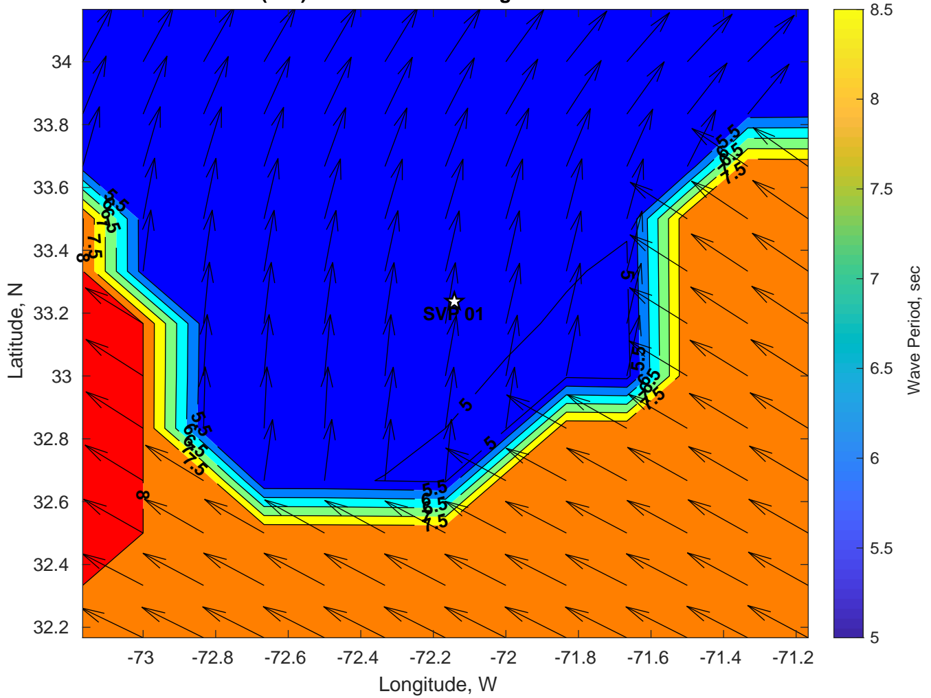
Wave Period (sec) for SVP 01 at 04-Aug-2024 06:00:00
