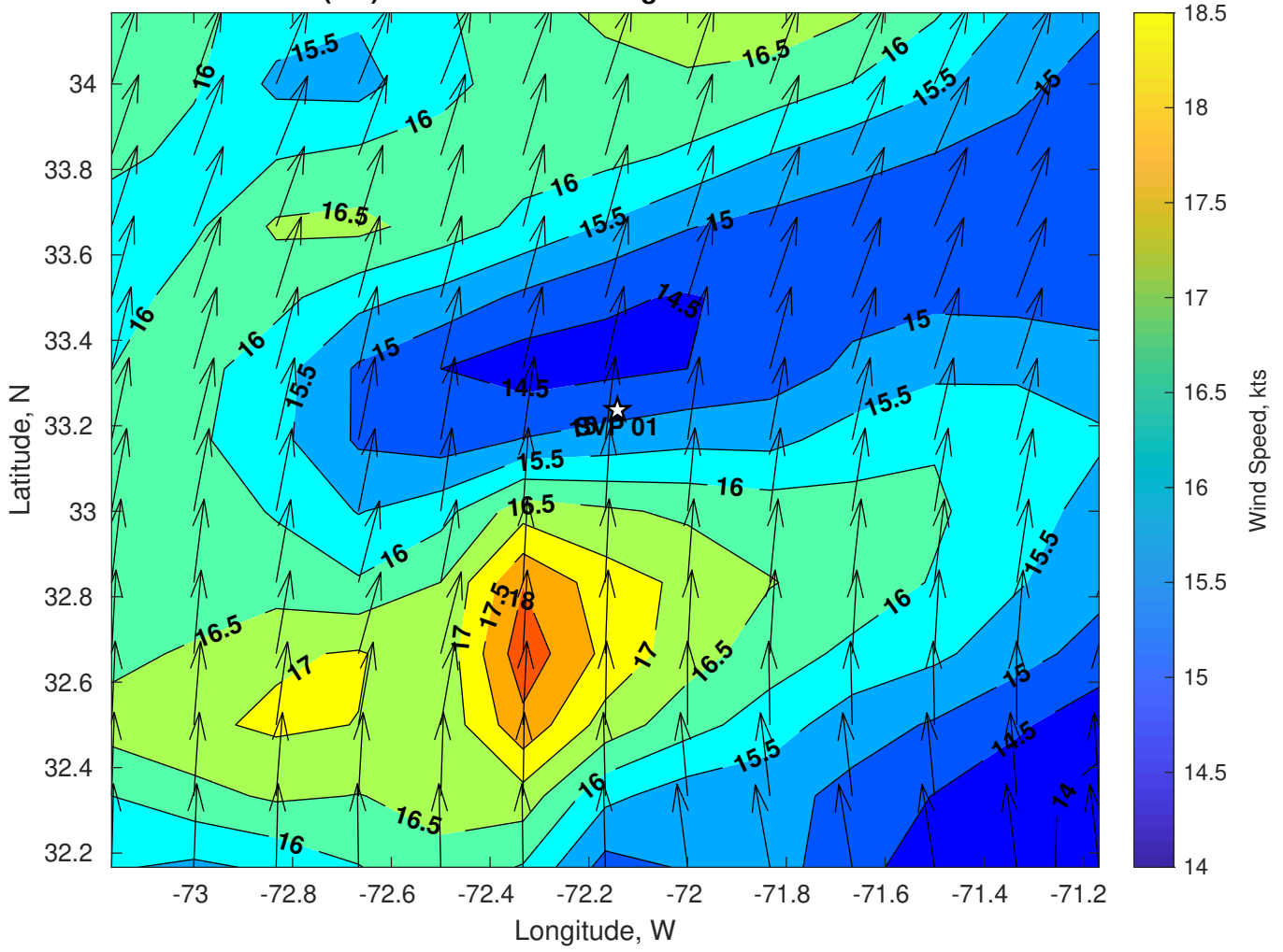
Winds (kts) for SVP 01 at 04-Aug-2024 06:00:00
