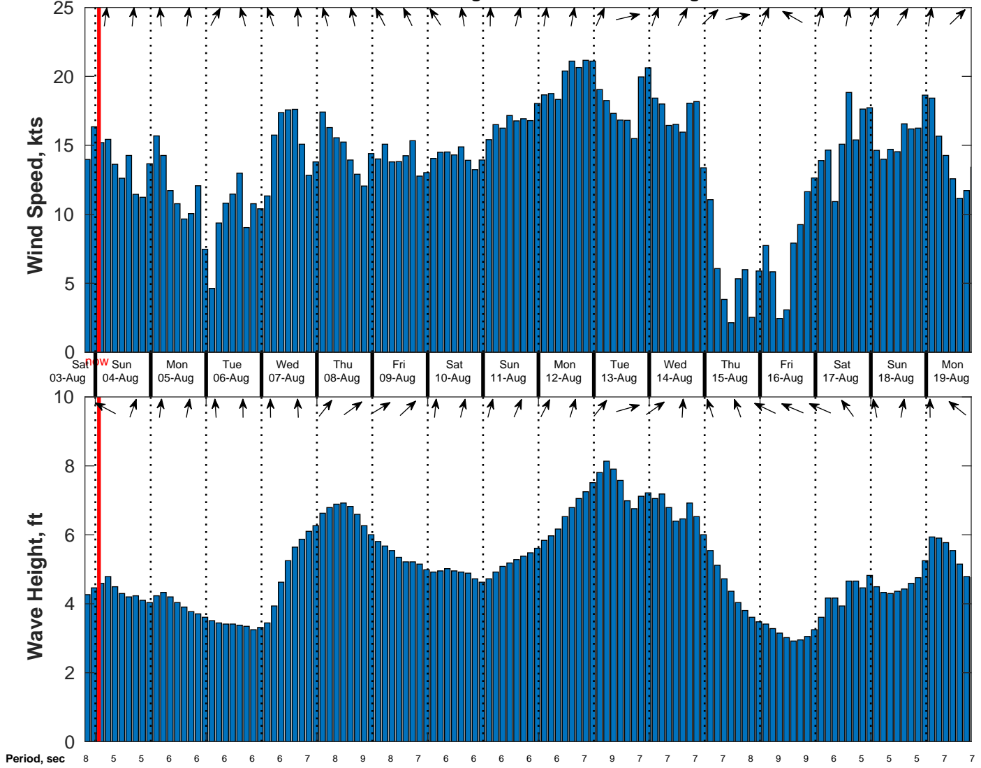
Wind & Wave Forecast for SVP 01 from 03-Aug-2024 19:00:00 to 19-Aug-2024 19:00:00
