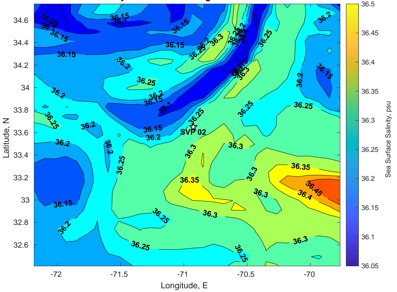
Surface Salinity for SVP 02 at 01-Aug-2024 00:00:00
