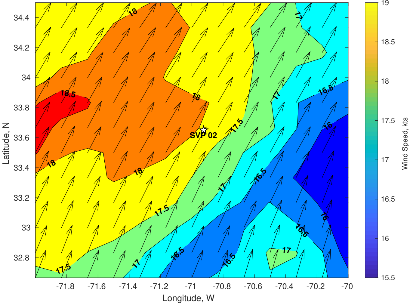
Winds (kts) for SVP 02 at 01-Aug-2024 06:00:00
