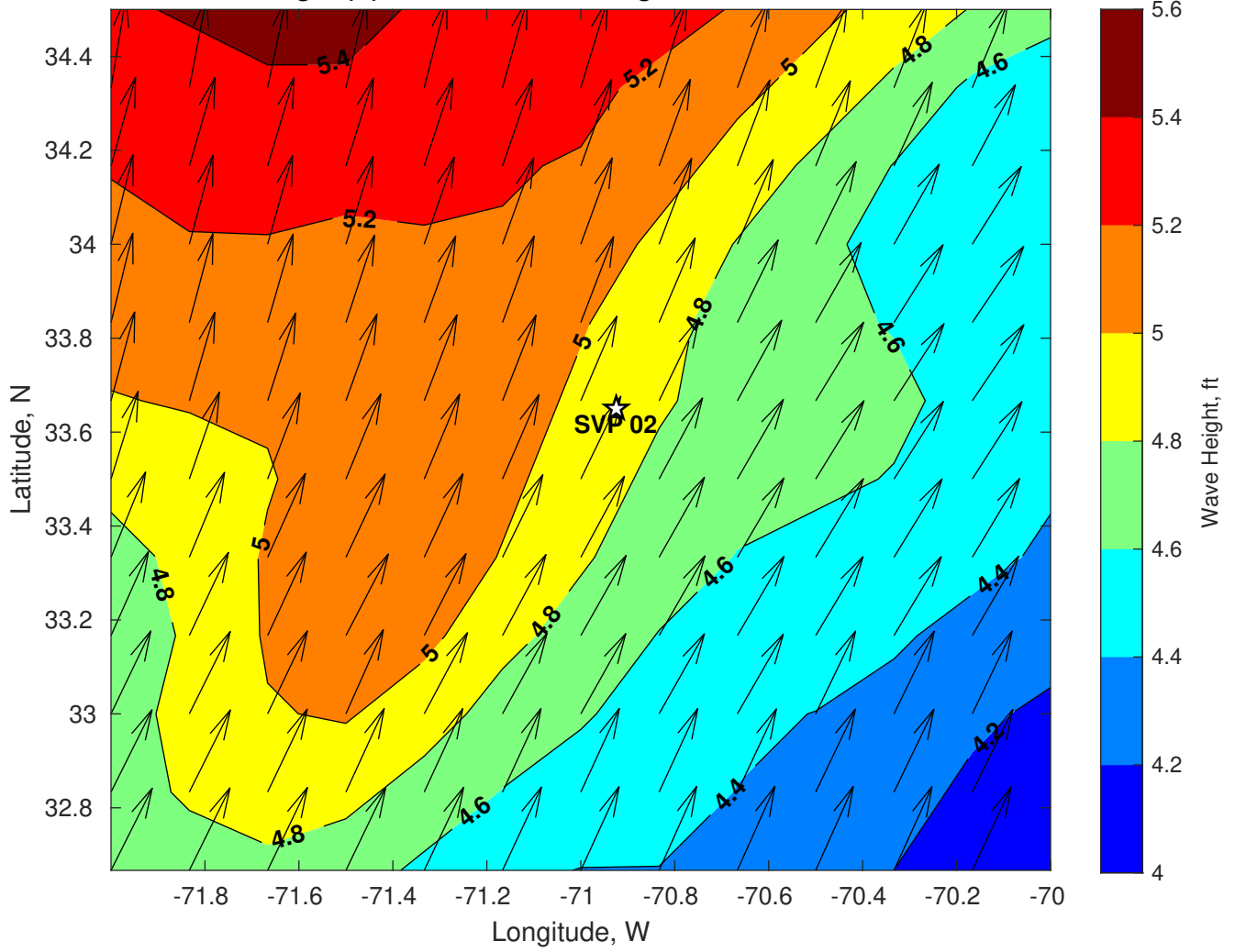
Wave Height (ft) for SVP 02 at 01-Aug-2024 06:00:00
