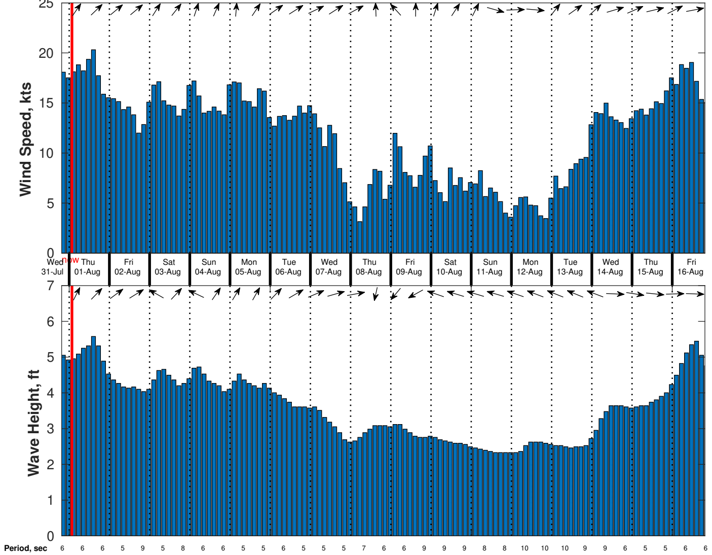
Wind & Wave Forecast for SVP 02 from 31-Jul-2024 19:00:00 to 16-Aug-2024 19:00:00
