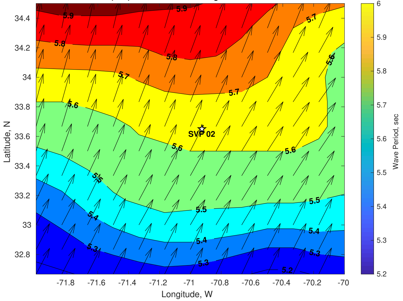
Wave Period (sec) for SVP 02 at 01-Aug-2024 06:00:00
