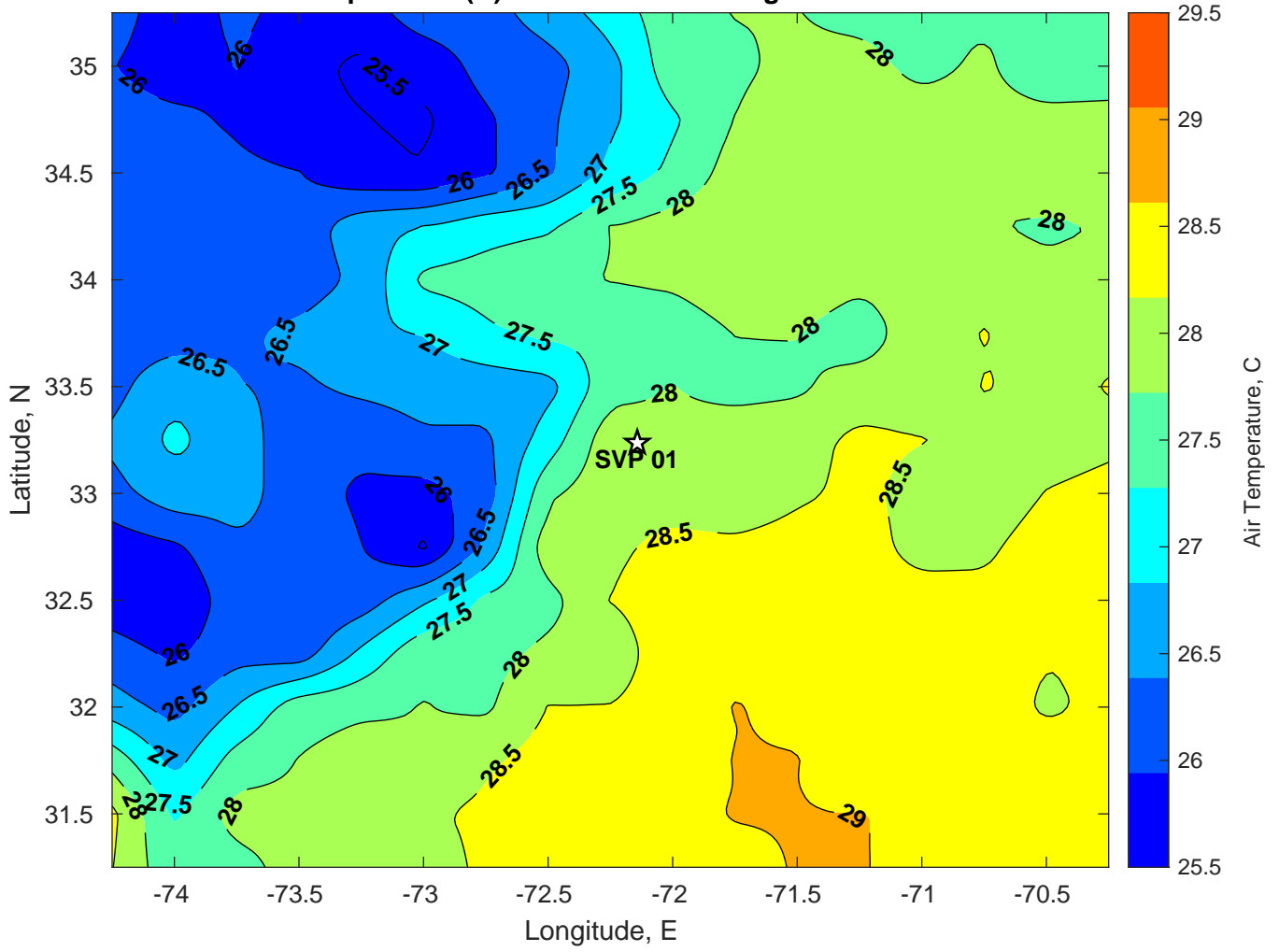
Air Temperature (C) for SVP 01 at 05-Aug-2024
