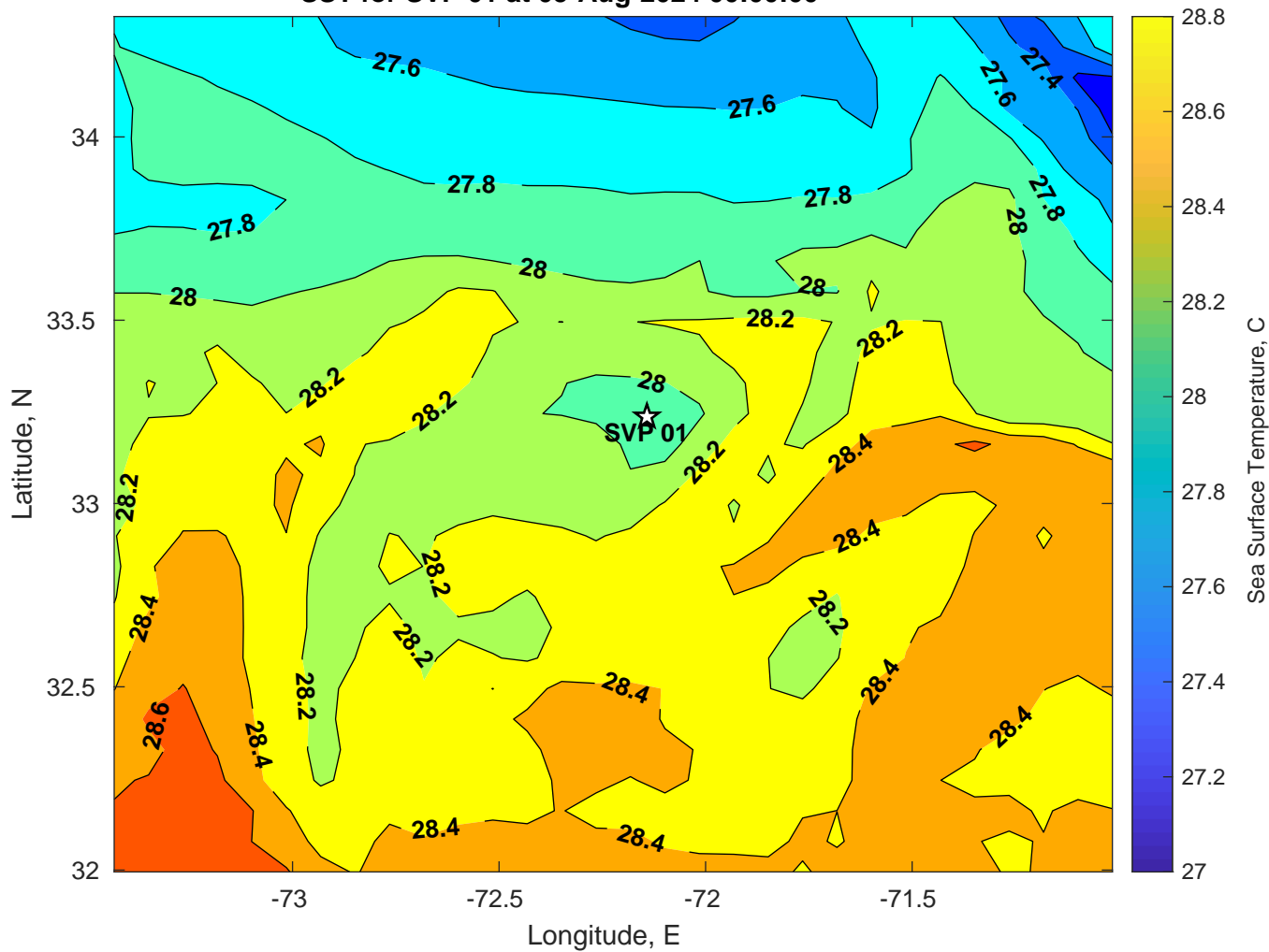
SST for SVP 01 at 05-Aug-2024 00:00:00
