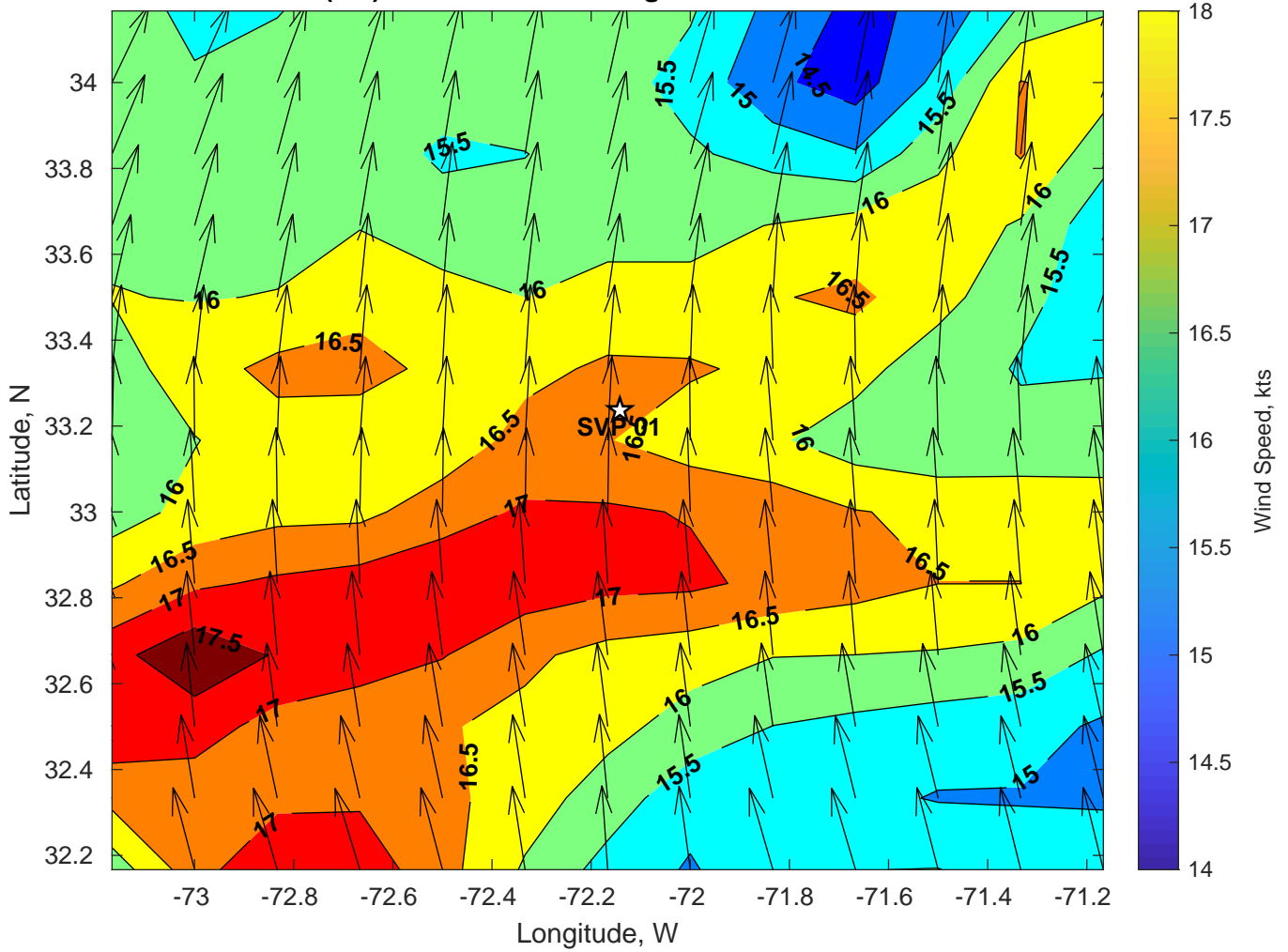
Winds (kts) for SVP 01 at 05-Aug-2024 06:00:00
