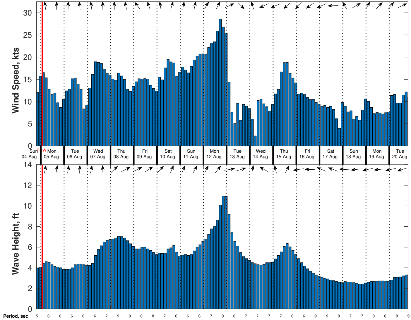
Wind & Wave Forecast for SVP 01 from 04-Aug-2024 19:00:00 to 20-Aug-2024 19:00:00
