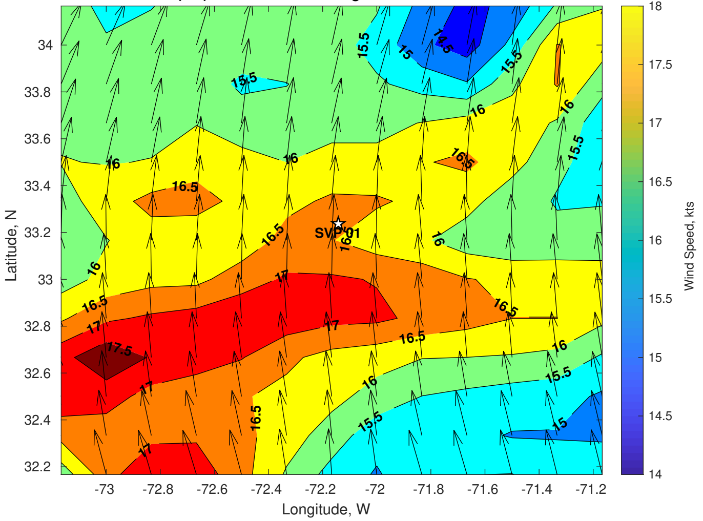
Winds (kts) for SVP 01 at 05-Aug-2024 06:00:00
