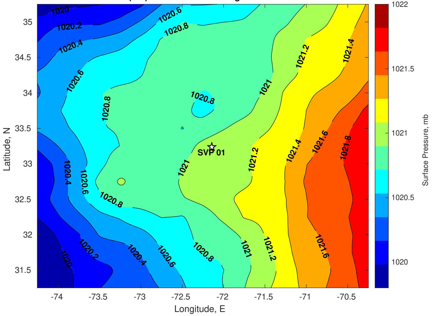
Surface Pressure (mb) for SVP 01 at 06-Aug-2024 00:00:00
