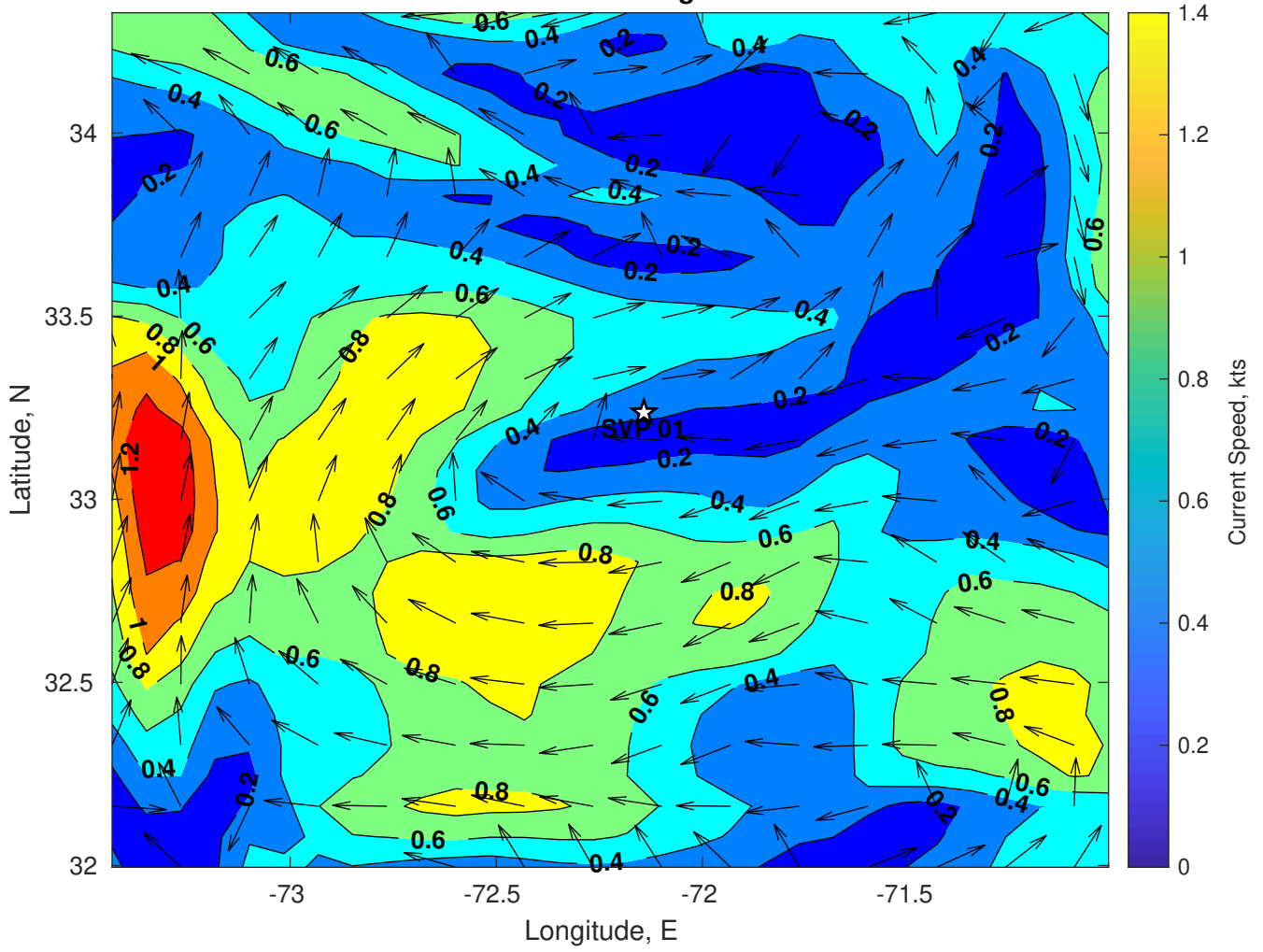
Surface Currents for SVP 01 at 05-Aug-2024 00:00:00
