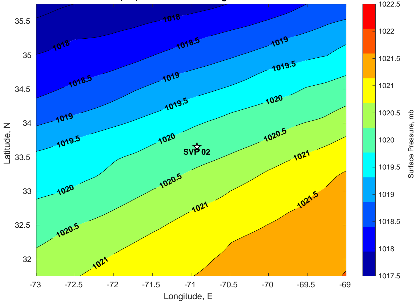
Surface Pressure (mb) for SVP 02 at 02-Aug-2024 00:00:00
