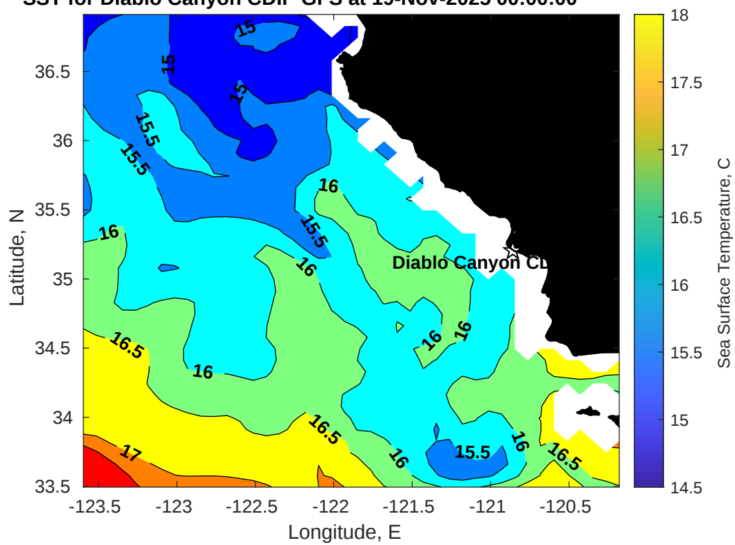
SST for Diablo Canyon CDIP GFS at 19-Nov-2025 00:00:00
