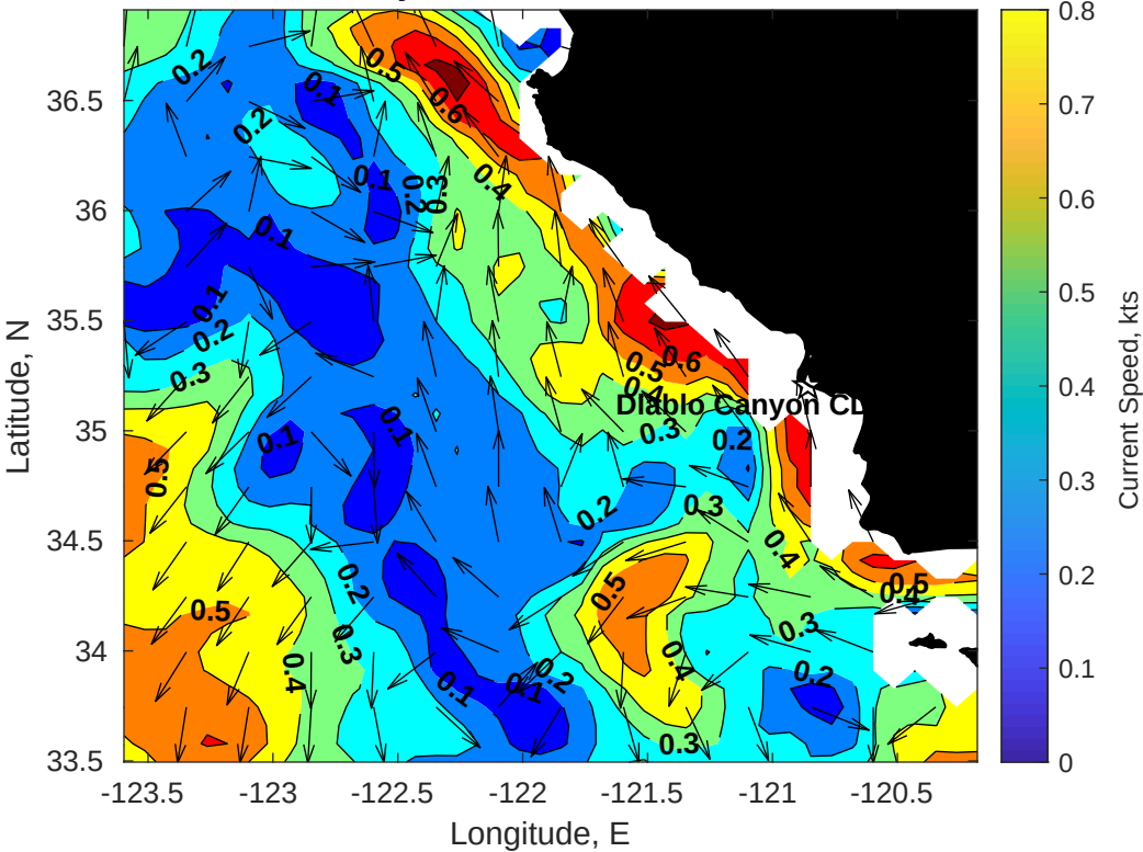
Surface Currents for Diablo Canyon CDIP GFS at 19-Nov-2025 00:00:00
