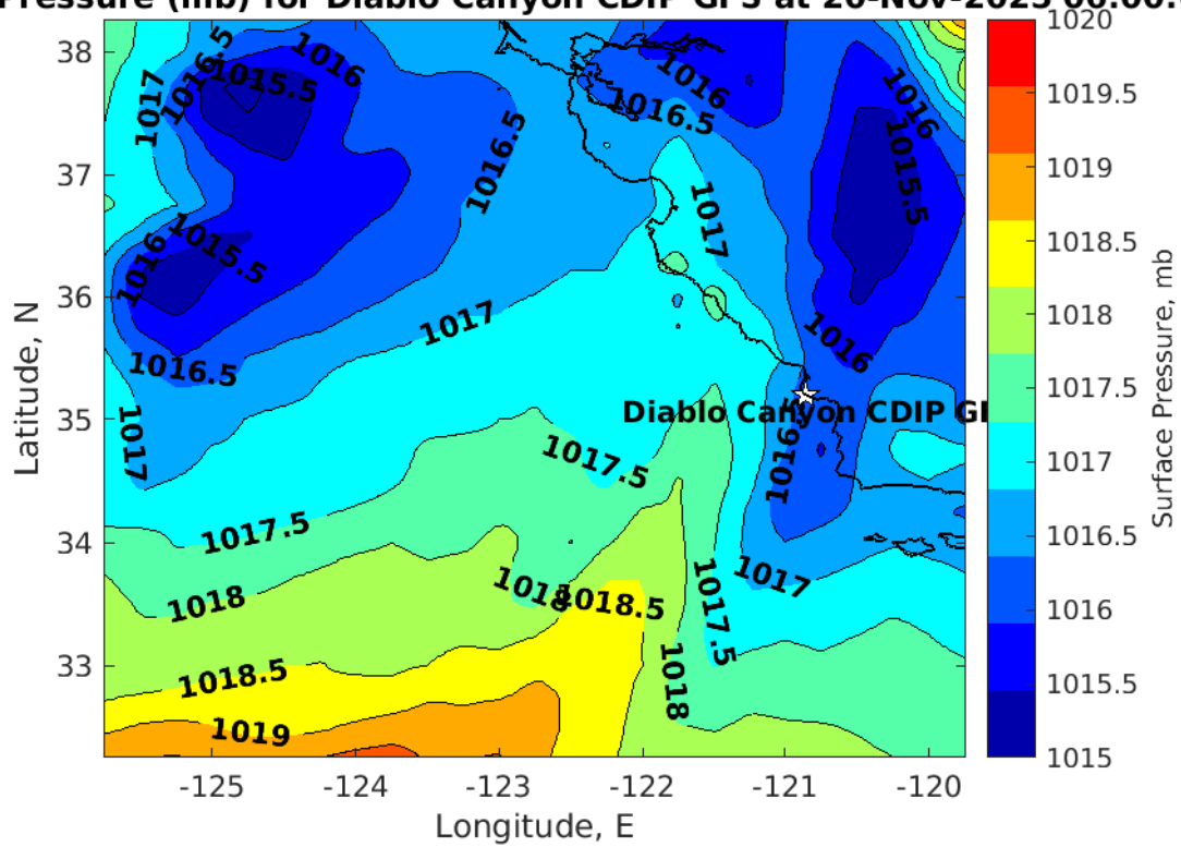
Surface Pressure (mb) for Diablo Canyon CDIP GFS at 20-Nov-2025 06:00:00
