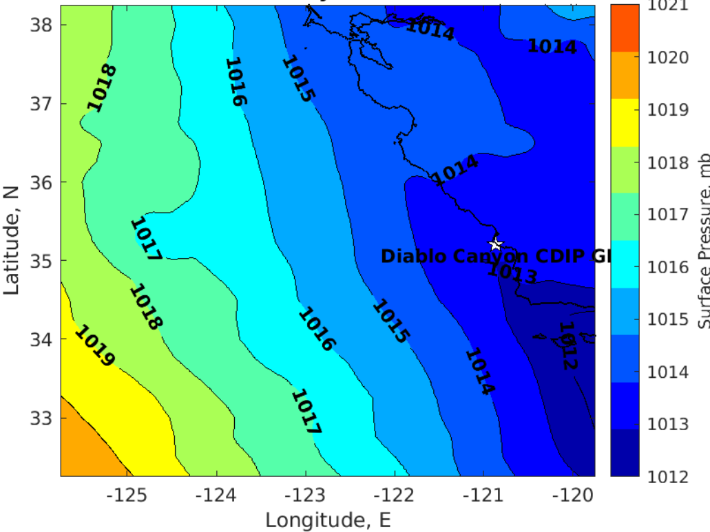
Surface Pressure (mb) for Diablo Canyon CDIP GFS at 21-Nov-2025 06:00:00
