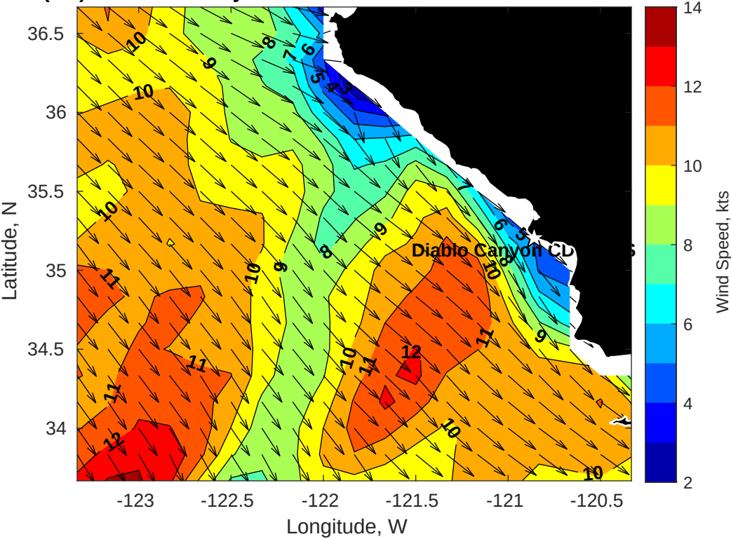
Winds (kts) for Diablo Canyon CDIP GFS at 19-Nov-2025 18:00:00
