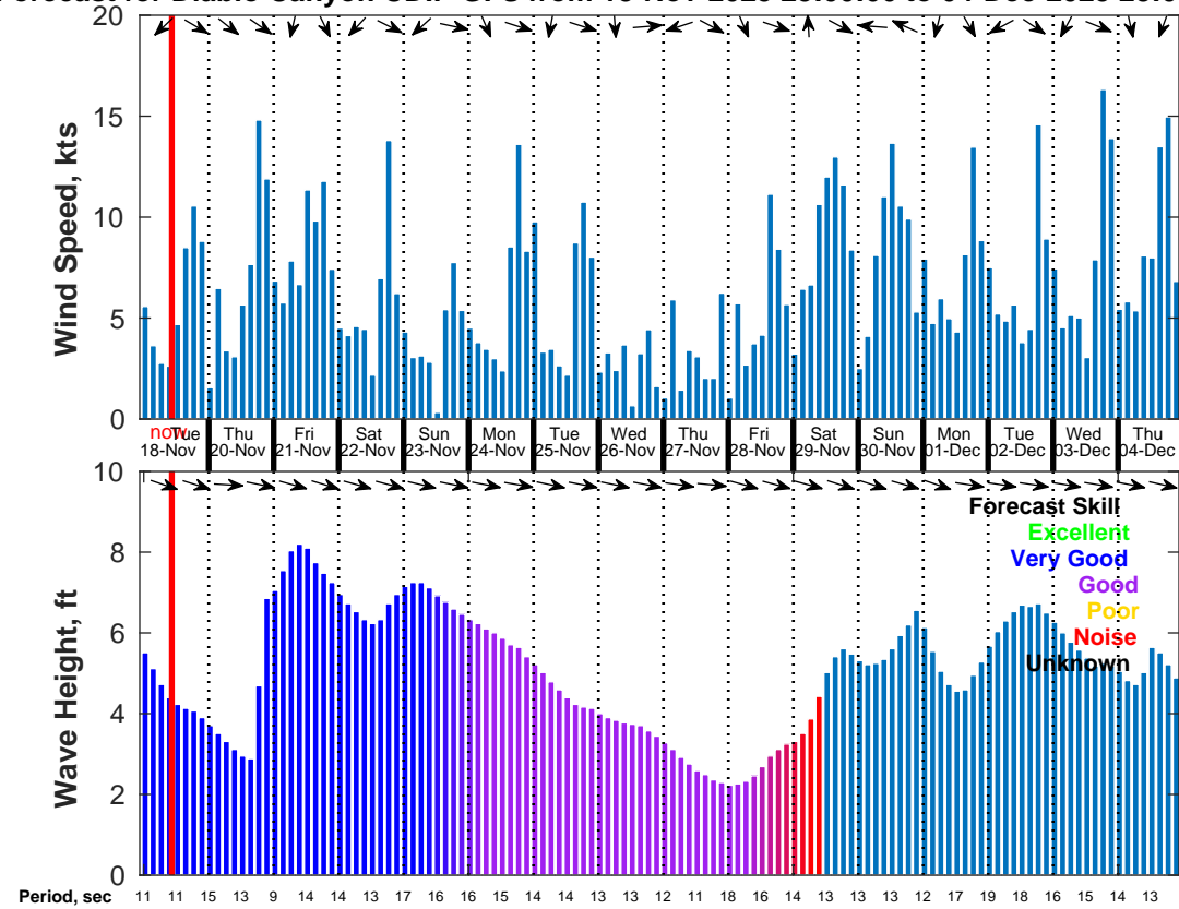
Wind & Wave Forecast for Diablo Canyon CDIP GFS from 18-Nov-2025 23:00:00 to 04-Dec-2025 23:00:00
