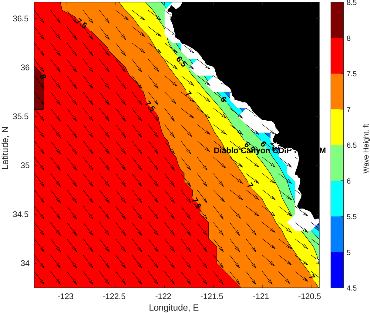
Wave Height (ft) for Diablo Canyon CDIP MFWAM at 19-Nov-2025 18:00:00
