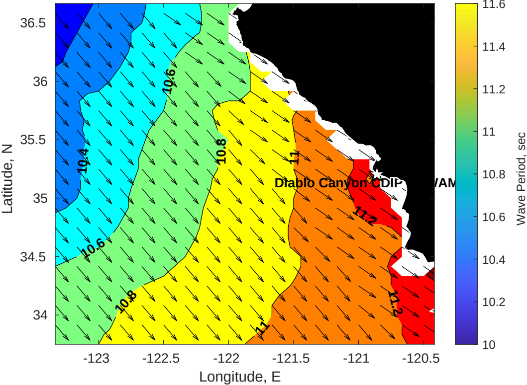
Wave Period (sec) for Diablo Canyon CDIP MFWAM at 19-Nov-2025 18:00:00
