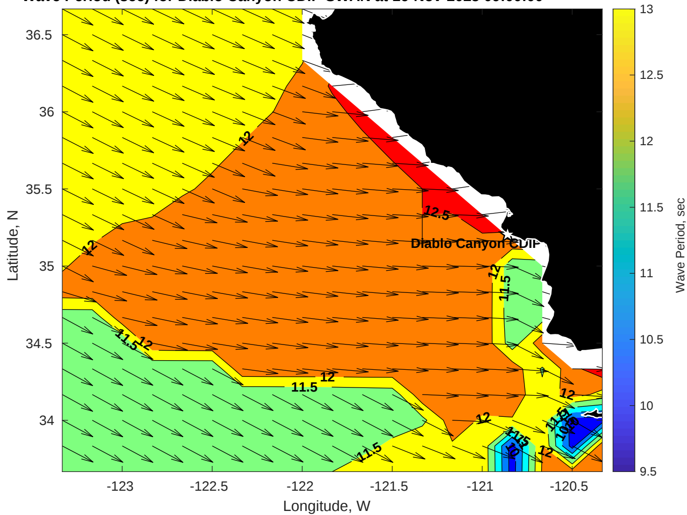
Wave Period (sec) for Diablo Canyon CDIP SWAN at 16-Nov-2025 09:00:00
