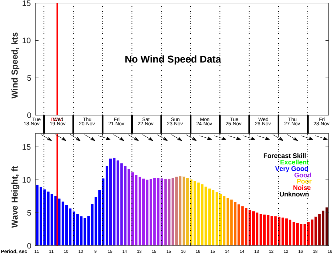
Wind & Wave Forecast for NDBC 46011 MFWAM from 18-Nov-2025 17:00:00 to 28-Nov-2025 17:00:00
