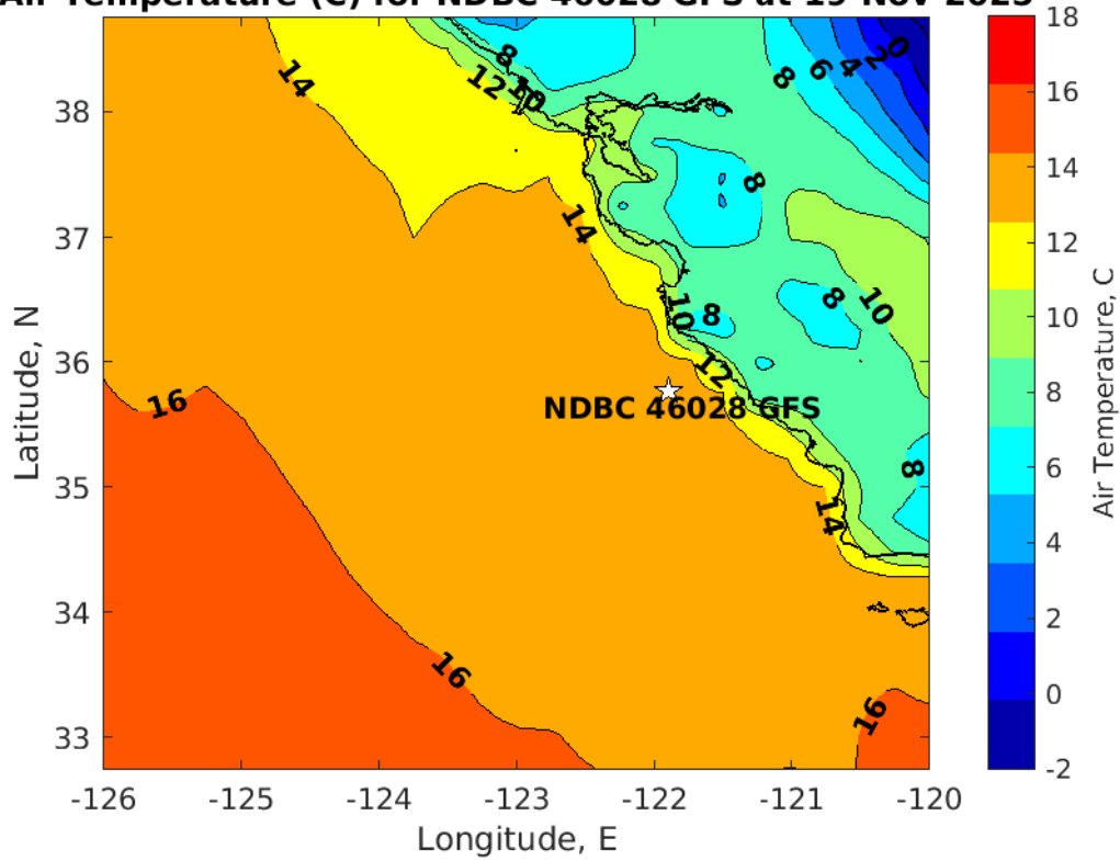
Air Temperature (C) for NDBC 46028 GFS at 19-Nov-2025
