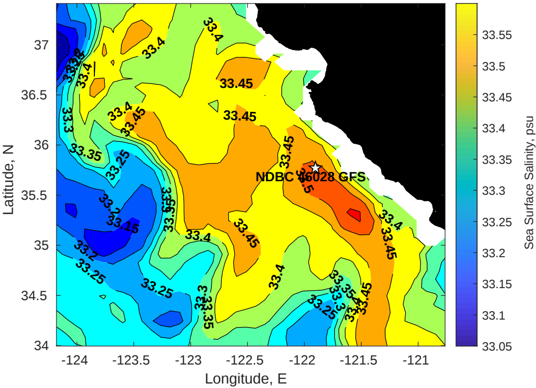
Surface Salinity for NDBC 46028 GFS at 19-Nov-2025 00:00:00
