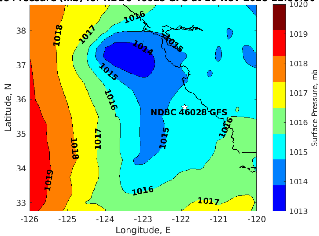
Surface Pressure (mb) for NDBC 46028 GFS at 20-Nov-2025 12:00:00
