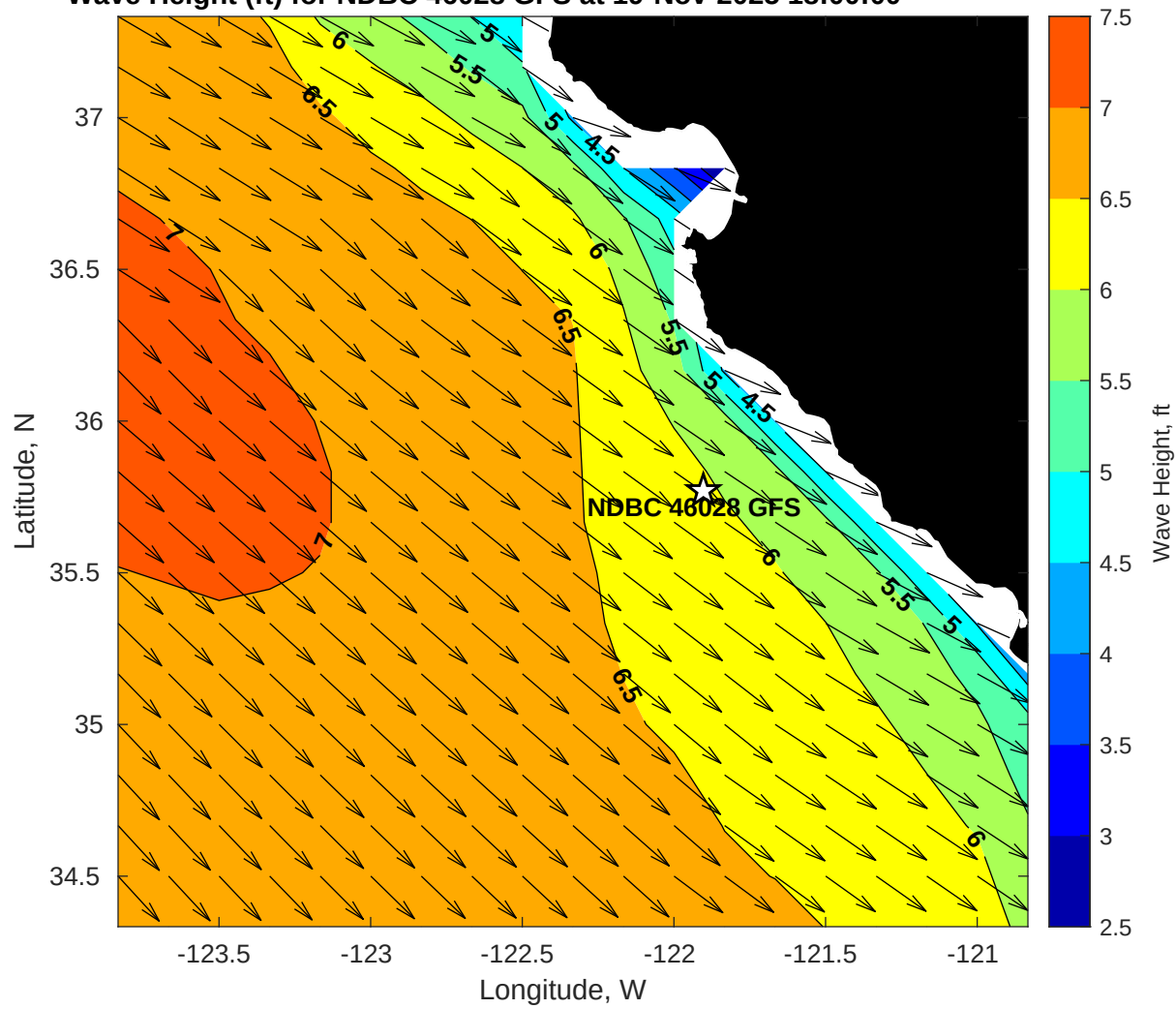
Wave Height (ft) for NDBC 46028 GFS at 19-Nov-2025 18:00:00
