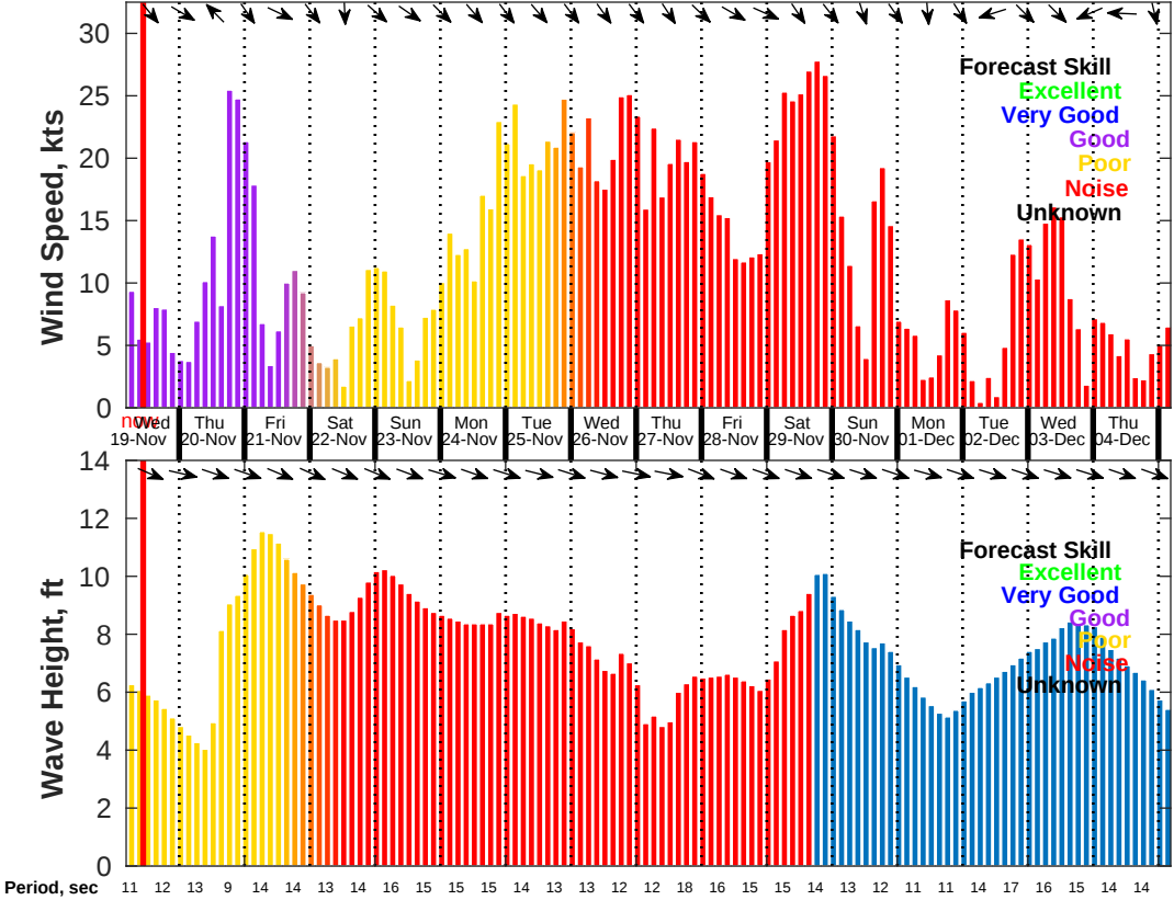
Wind & Wave Forecast for NDBC 46028 GFS from 19-Nov-2025 05:00:00 to 05-Dec-2025 05:00:00
