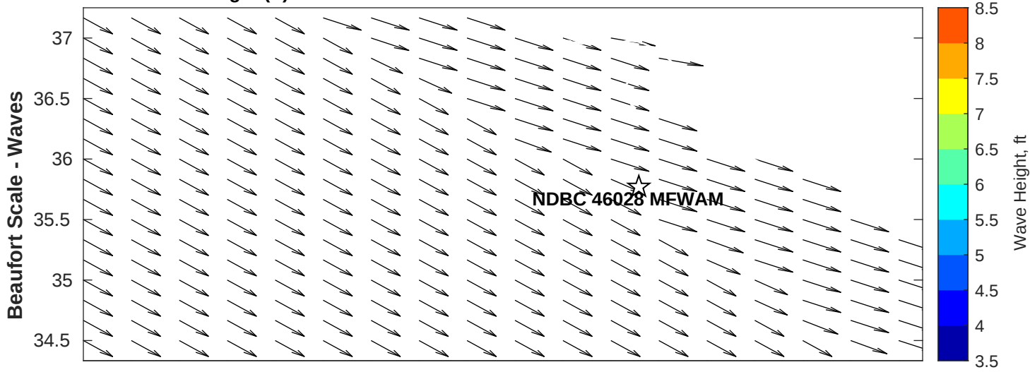
Wave Height (ft) for NDBC 46028 MFWAM at 19-Nov-2025 18:00:00
