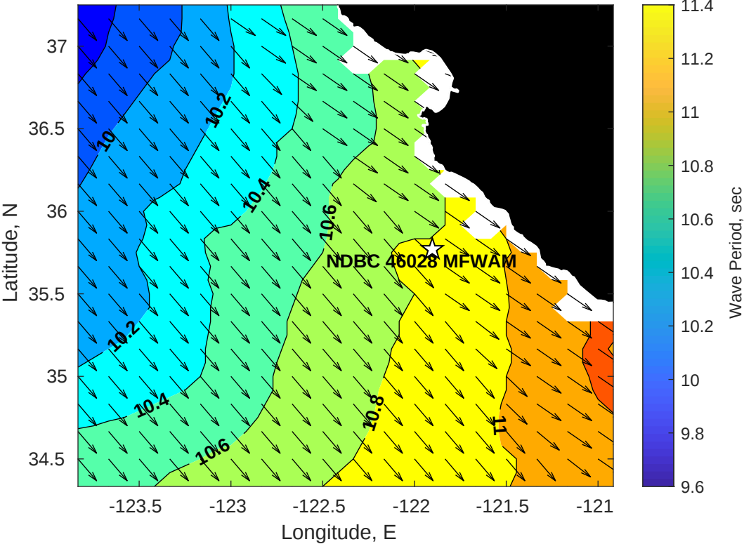
Wave Period (sec) for NDBC 46028 MFWAM at 19-Nov-2025 18:00:00
