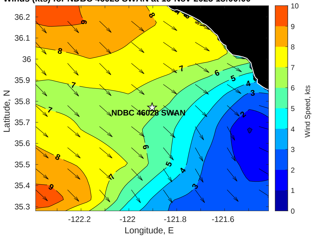
Winds (kts) for NDBC 46028 SWAN at 19-Nov-2025 18:00:00
