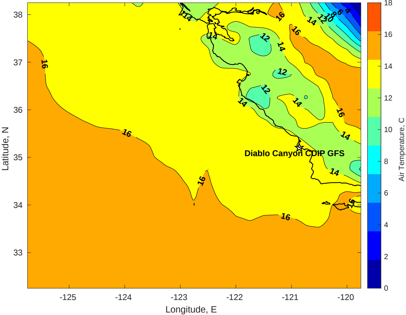
Air Temperature (C) for Diablo Canyon CDIP GFS at 20-Nov-2025
