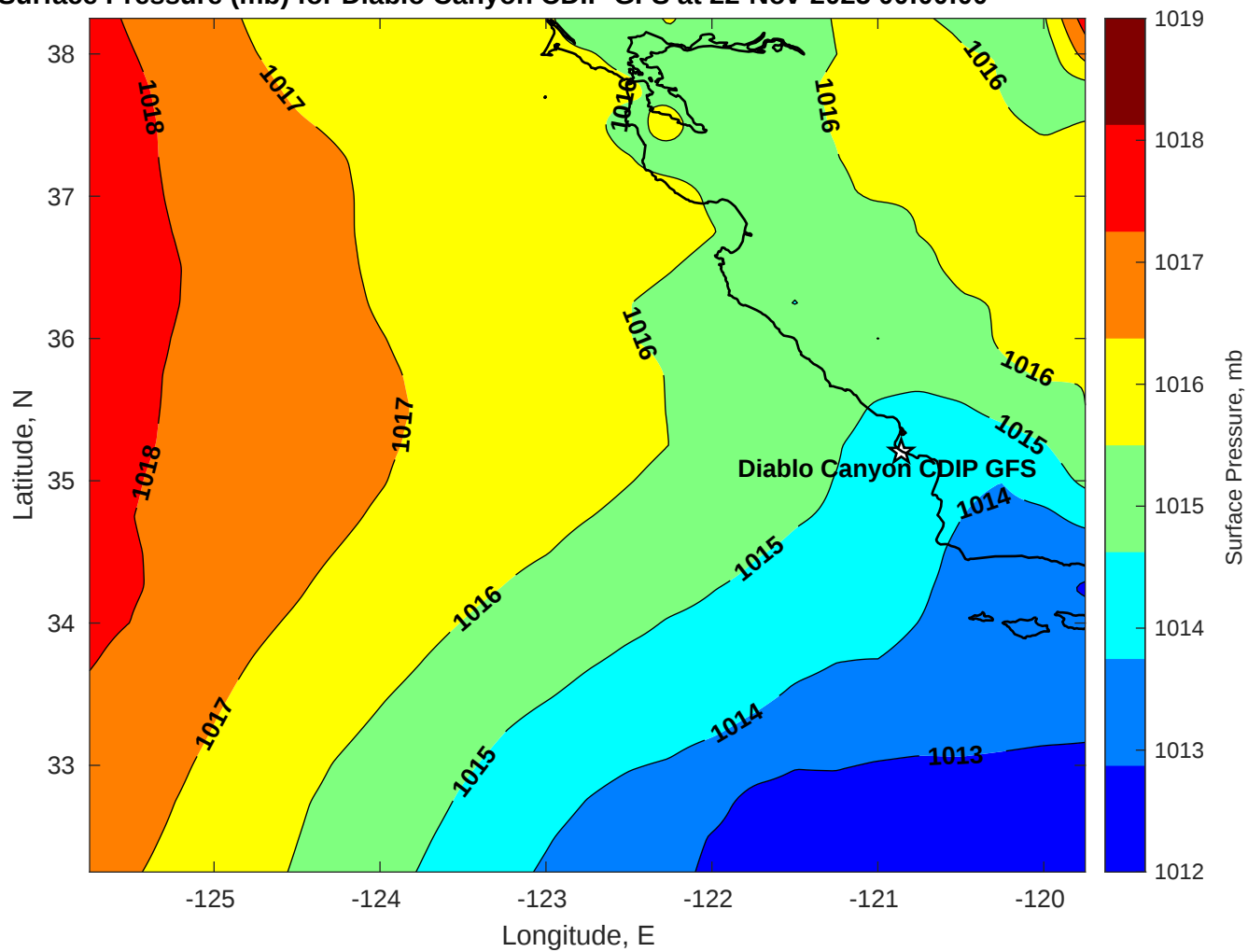
Surface Pressure (mb) for Diablo Canyon CDIP GFS at 22-Nov-2025 00:00:00
