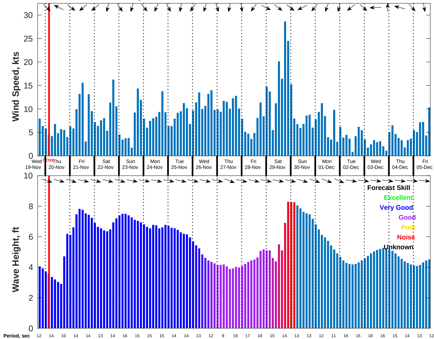
Wind & Wave Forecast for Diablo Canyon CDIP GFS from 19-Nov-2025 17:00:00 to 05-Dec-2025 17:00:00
