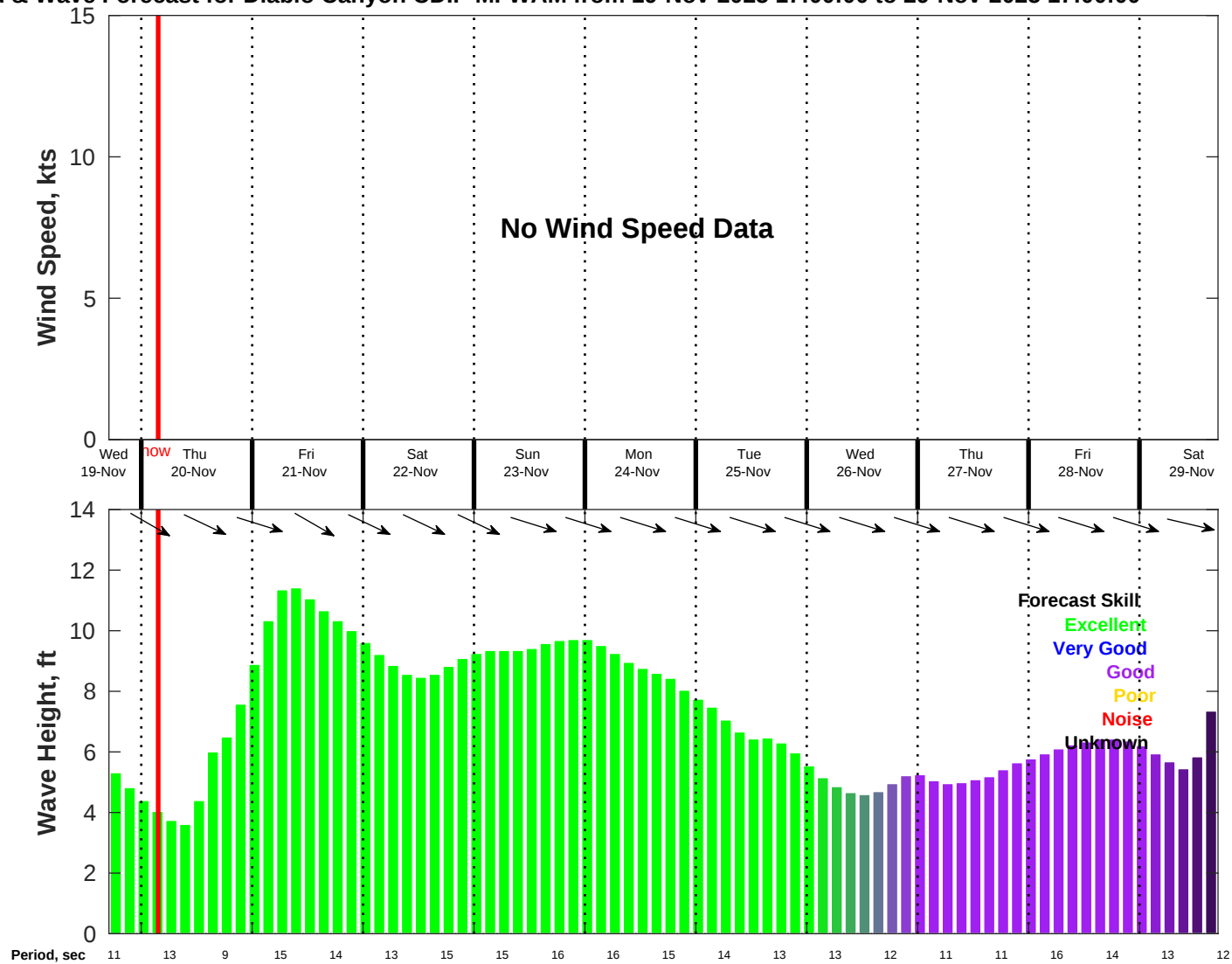
Wind & Wave Forecast for Diablo Canyon CDIP MFWAM from 19-Nov-2025 17:00:00 to 29-Nov-2025 17:00:00
