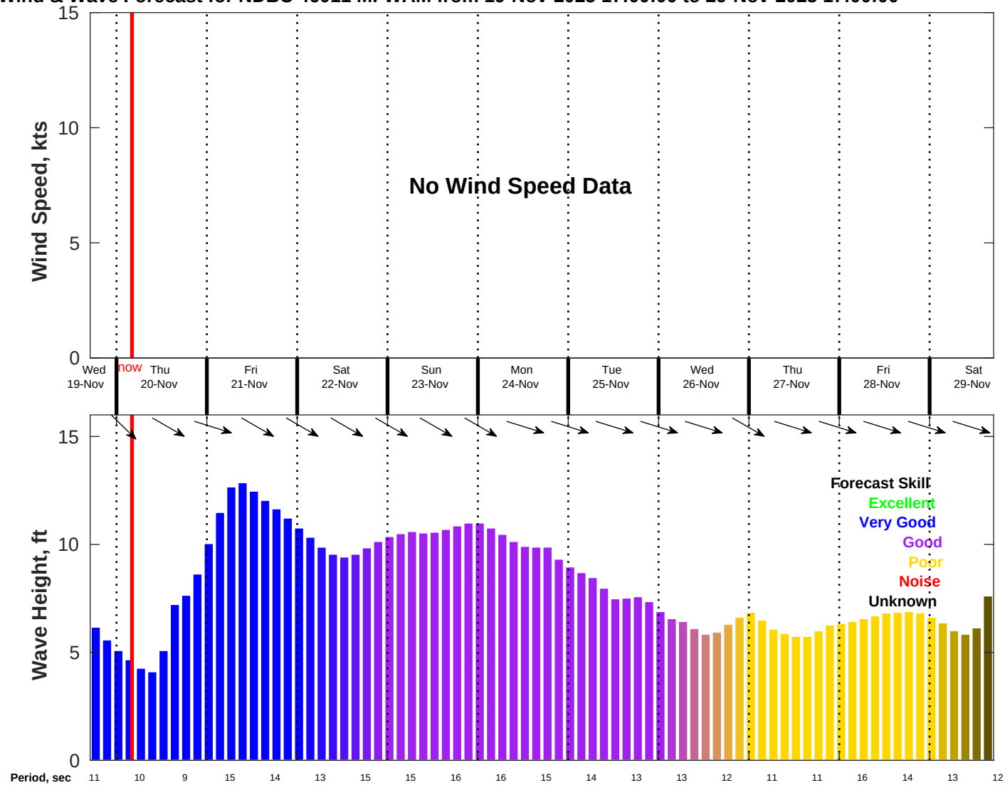
Wind & Wave Forecast for NDBC 46011 MFWAM from 19-Nov-2025 17:00:00 to 29-Nov-2025 17:00:00
