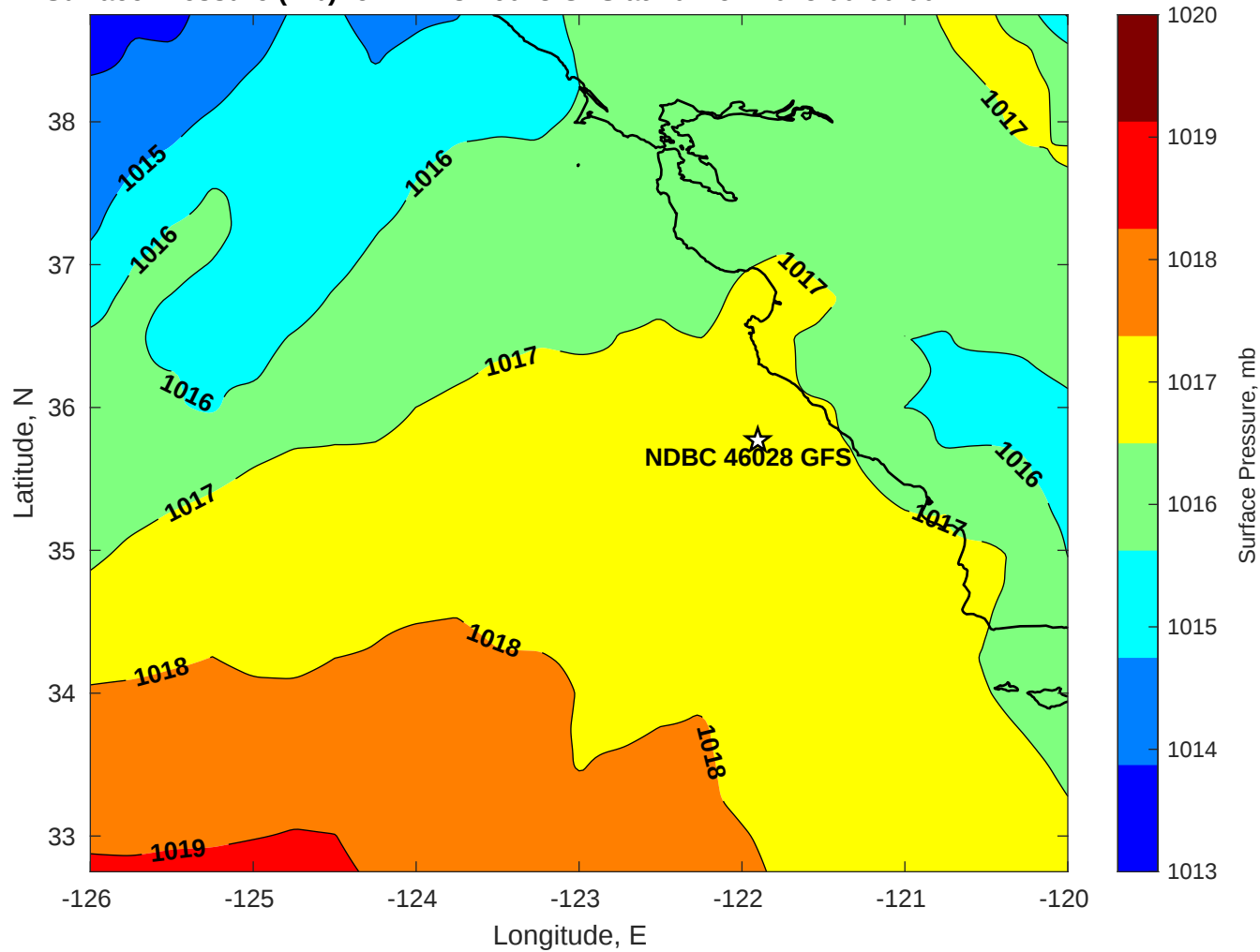
Surface Pressure (mb) for NDBC 46028 GFS at 20-Nov-2025 00:00:00
