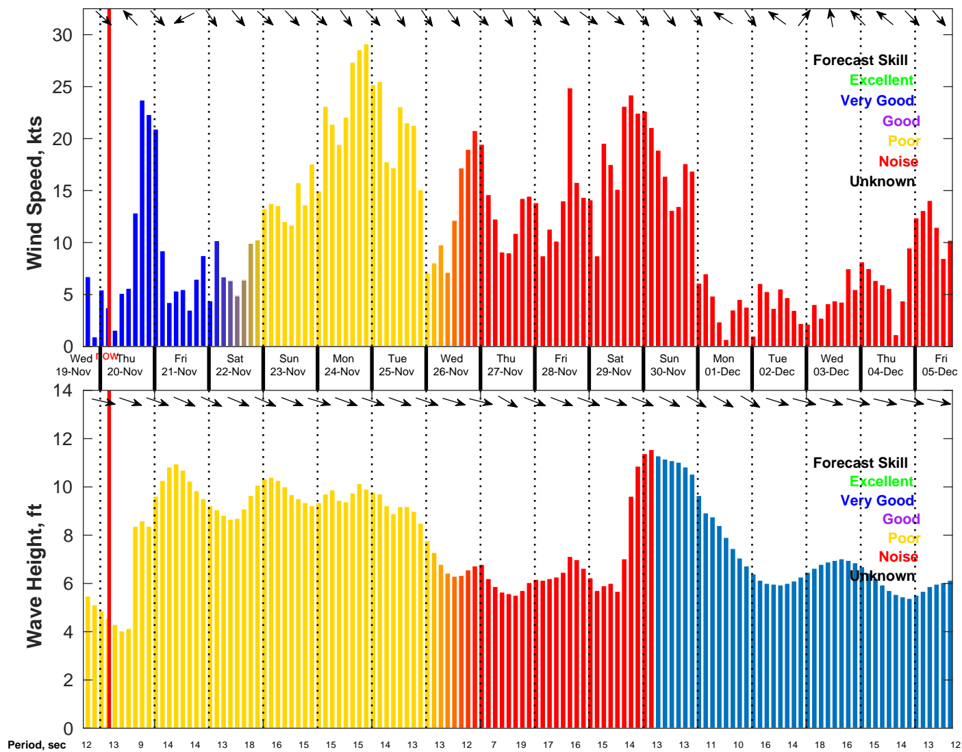
Wind & Wave Forecast for NDBC 46028 GFS from 19-Nov-2025 17:00:00 to 05-Dec-2025 17:00:00
