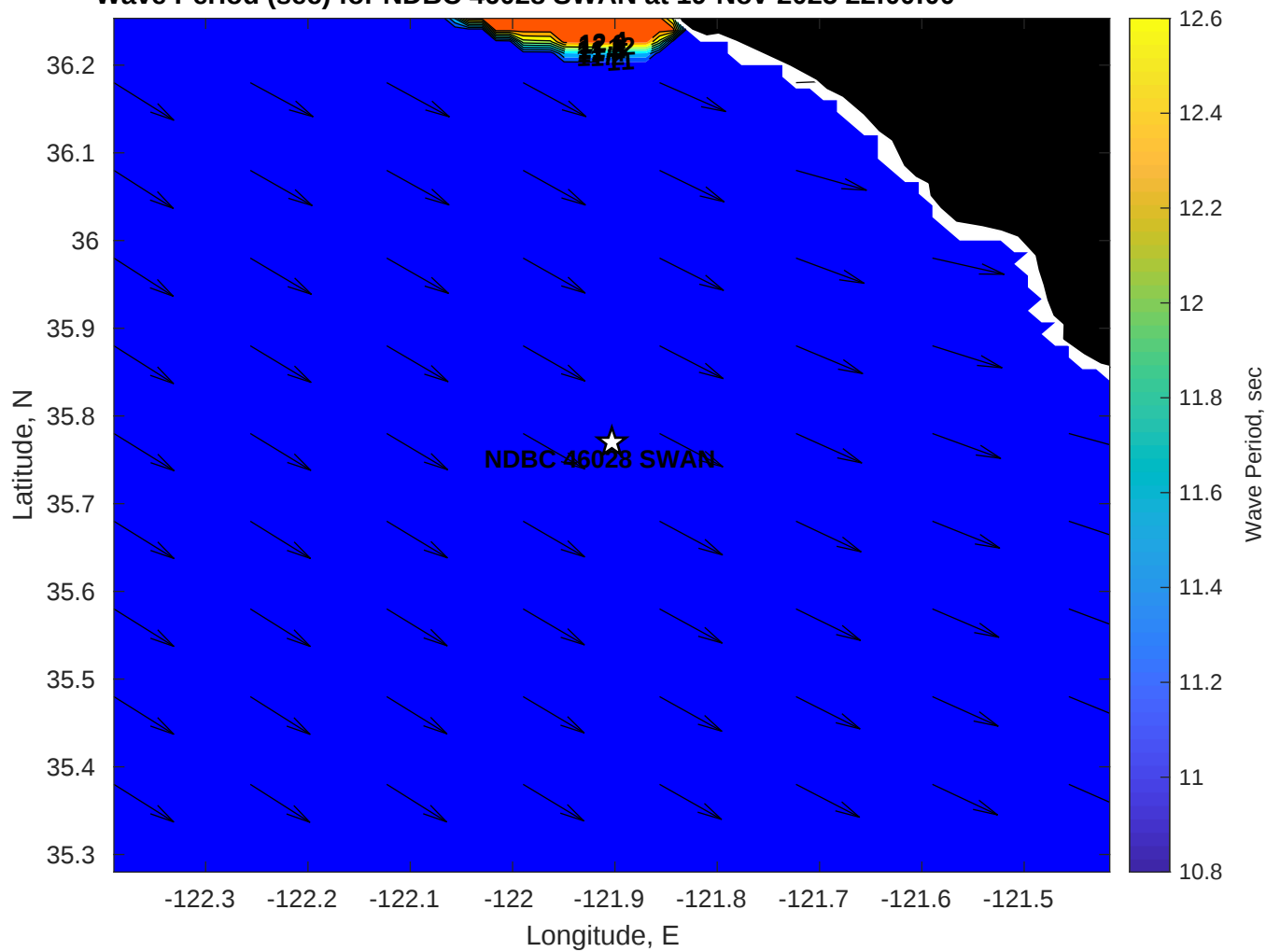
Wave Period (sec) for NDBC 46028 SWAN at 19-Nov-2025 22:00:00
