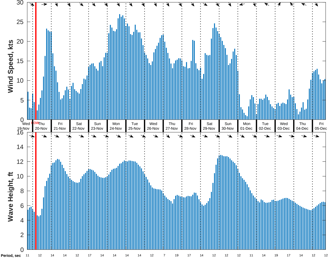
Wind & Wave Forecast for NDBC 46028 SWAN from 19-Nov-2025 17:00:00 to 05-Dec-2025 17:00:00
