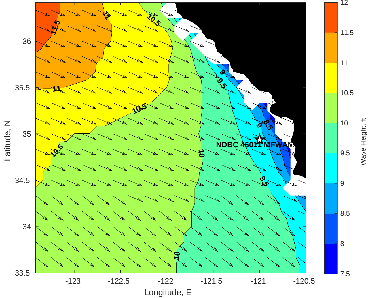
WAM Wave Height (ft) for NDBC 46011 MFWAM at 23-Nov-2025 09:00:00
