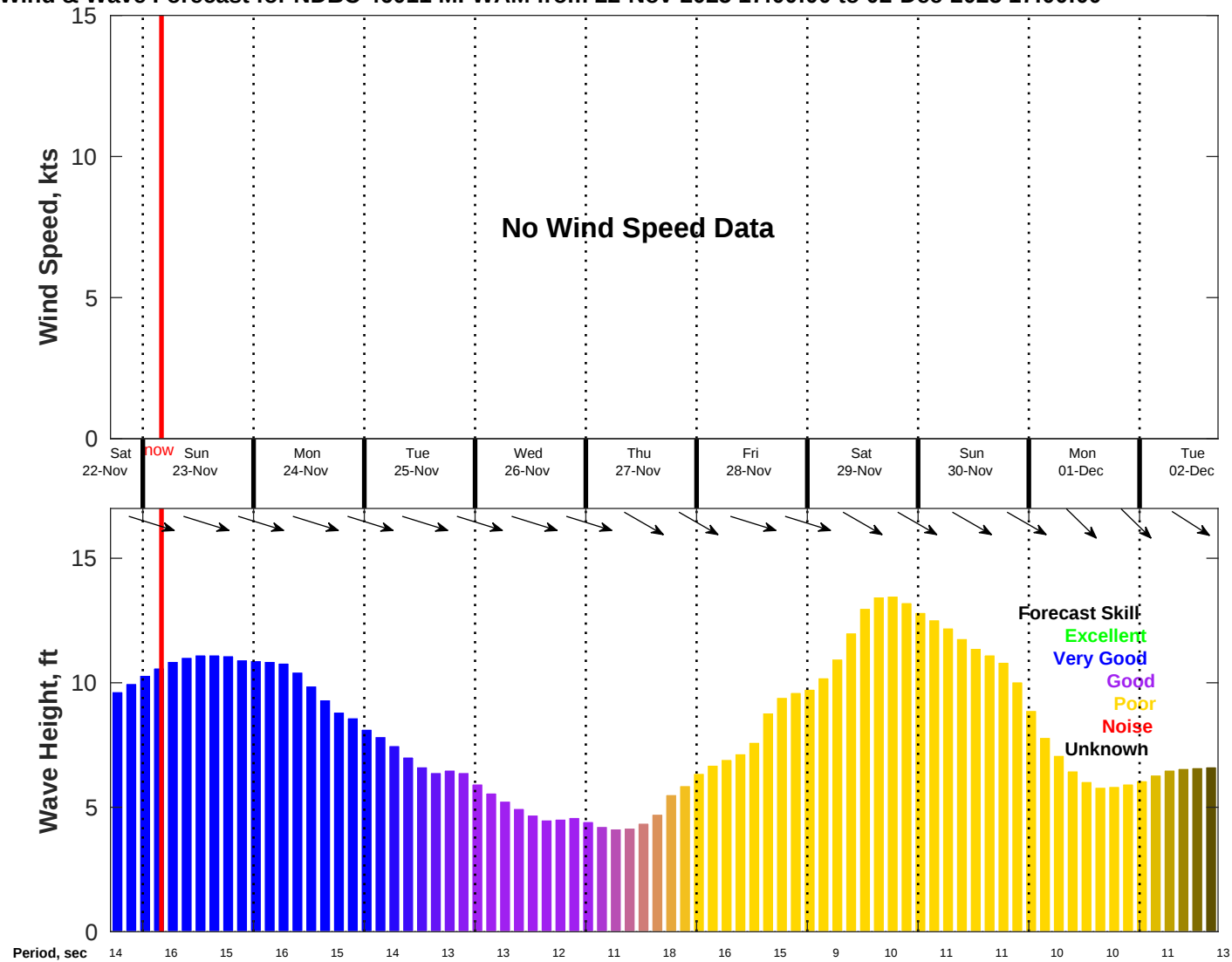
Wind & Wave Forecast for NDBC 46011 MFWAM from 22-Nov-2025 17:00:00 to 02-Dec-2025 17:00:00
