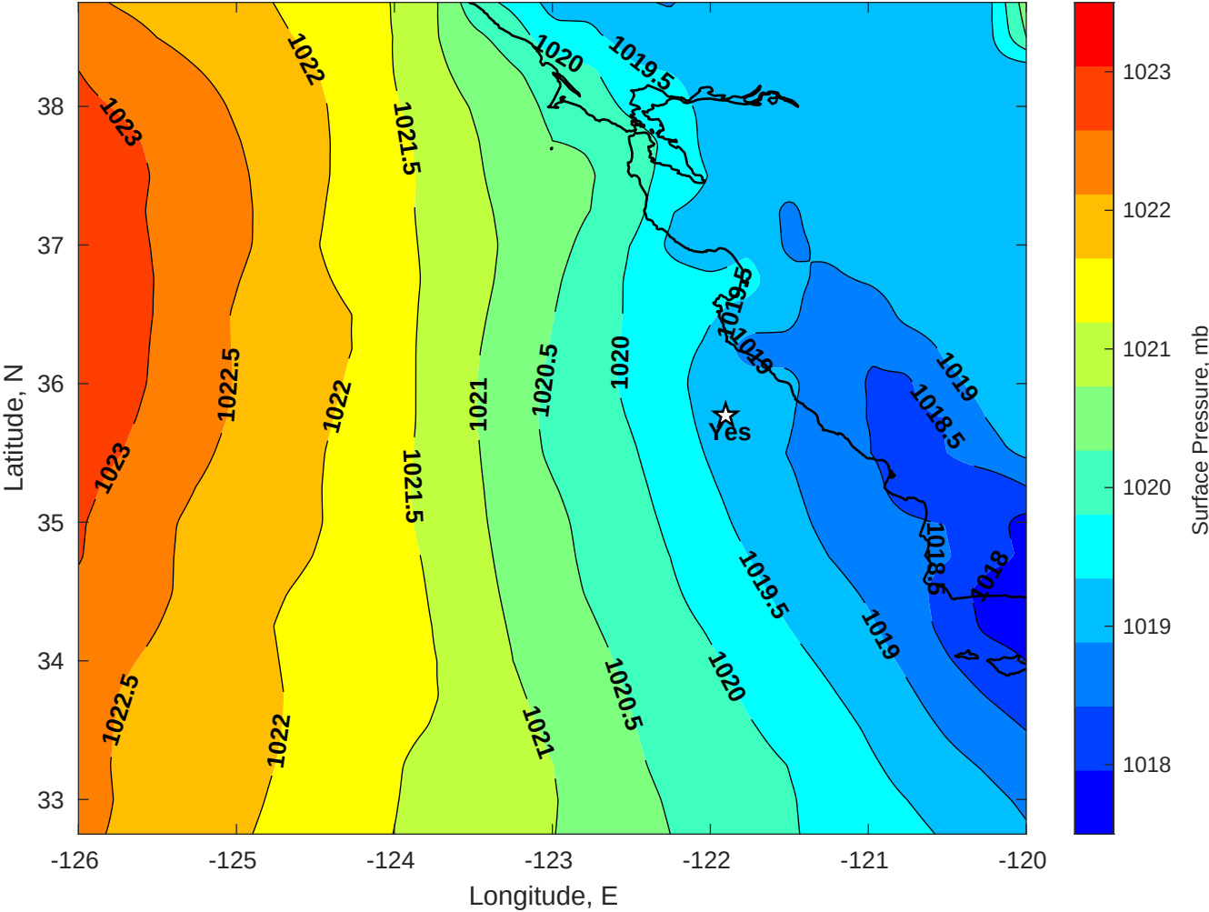
Surface Pressure (mb) for Yes at 24-Nov-2025 00:00:00
