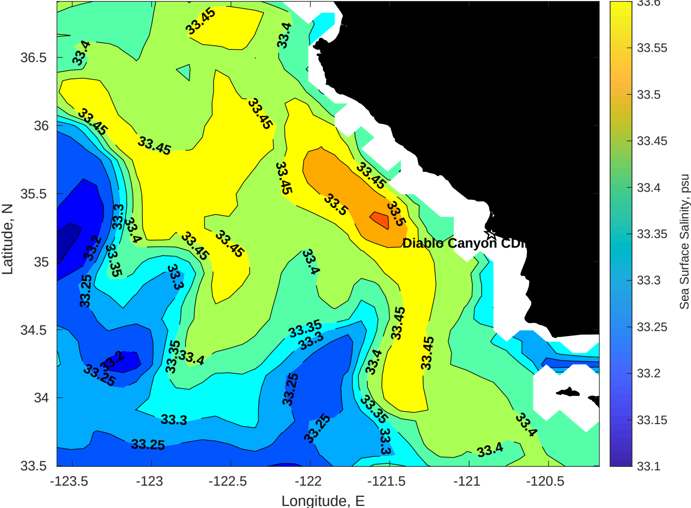
Surface Salinity for Diablo Canyon CDIP GFS at 19-Nov-2025 00:00:00
