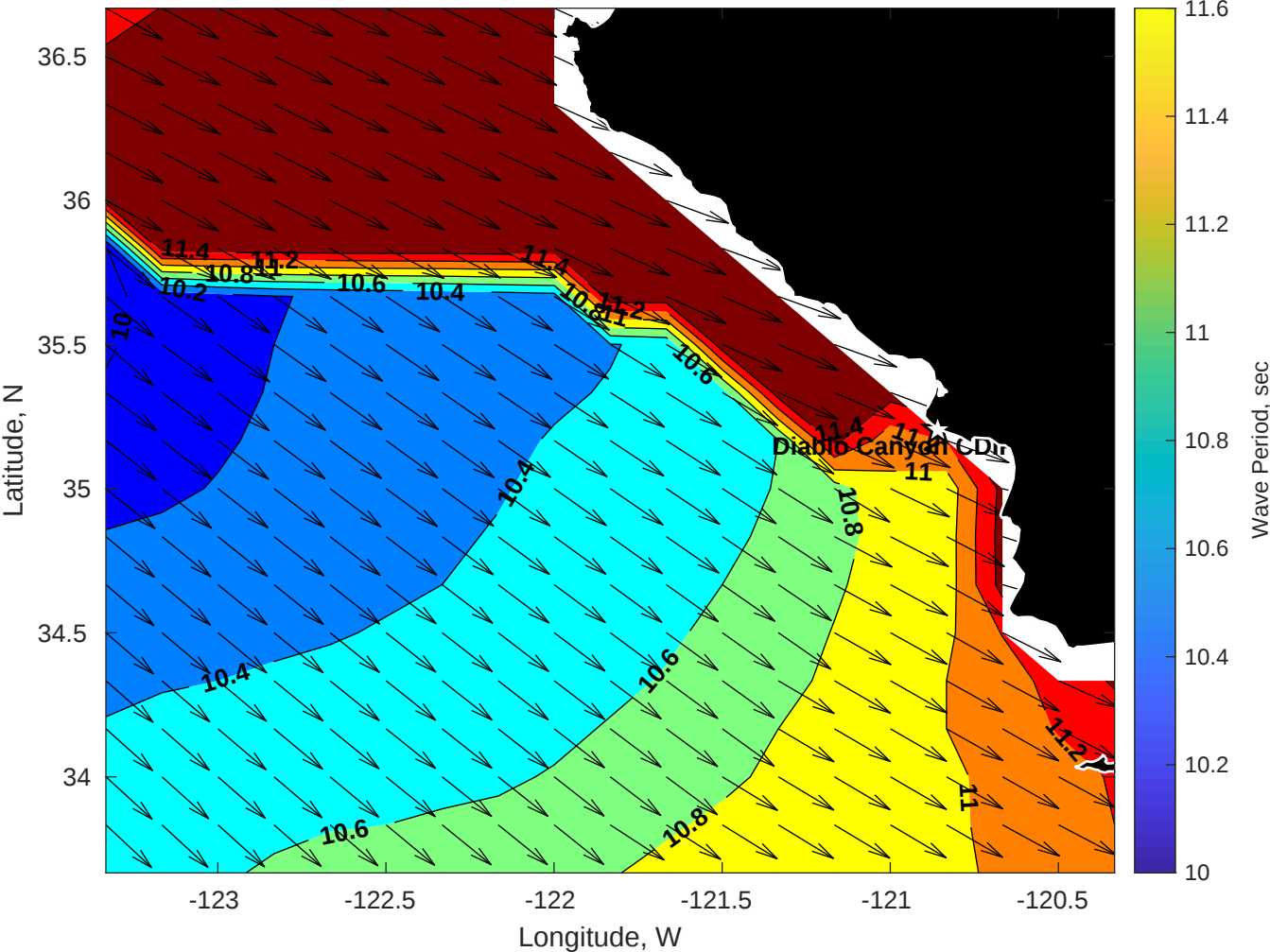
Wave Period (sec) for Diablo Canyon CDIP GFS at 19-Nov-2025 21:00:00
