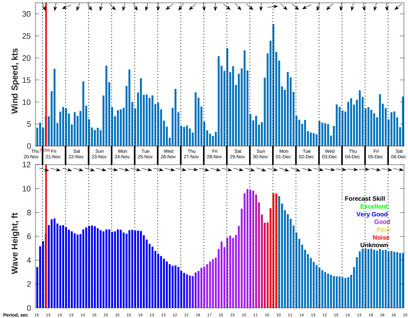
Wind & Wave Forecast for Diablo Canyon CDIP GFS from 20-Nov-2025 17:00:00 to 06-Dec-2025 17:00:00
