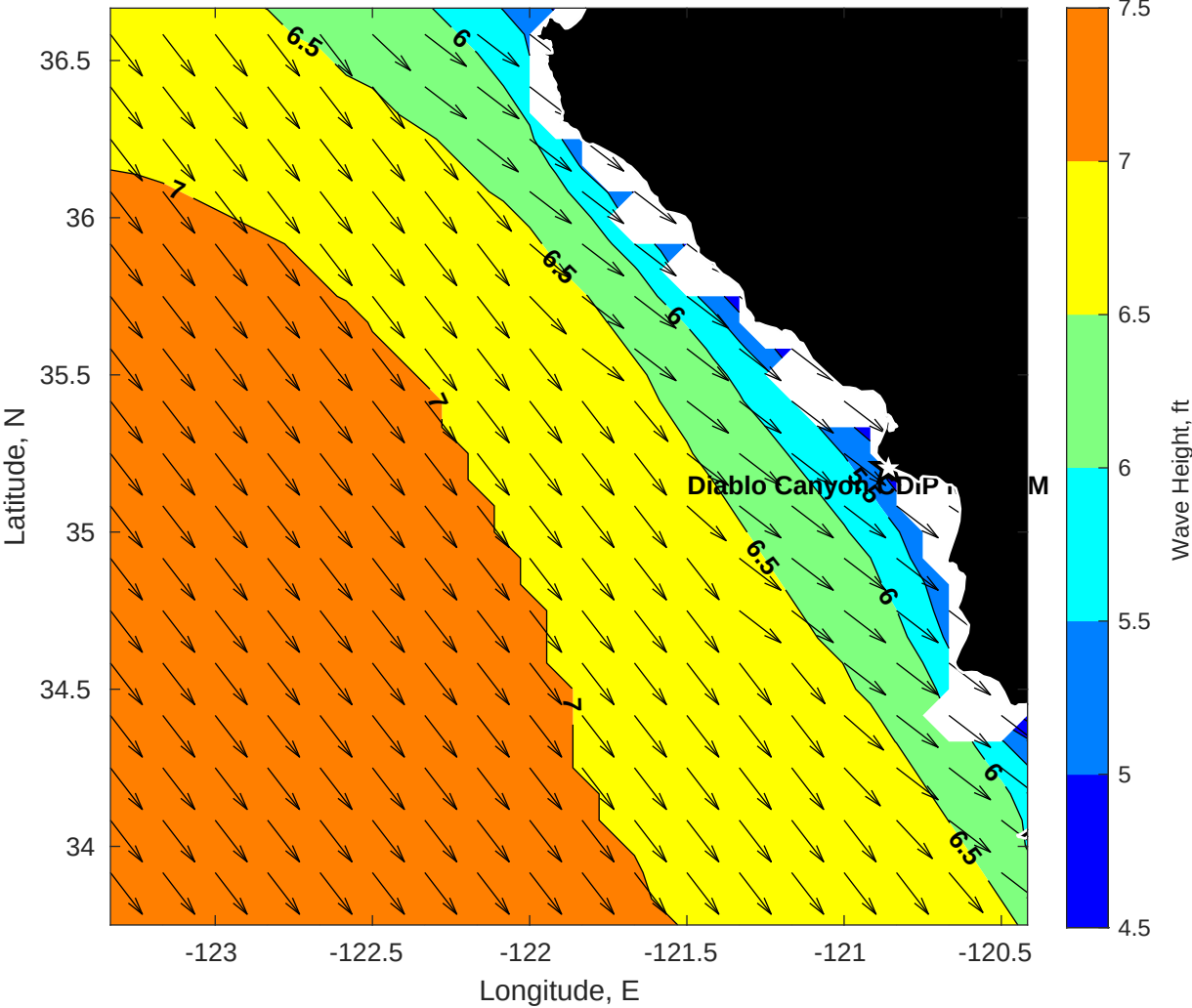
Wave Height (ft) for Diablo Canyon CDIP MFWAM at 19-Nov-2025 21:00:00
