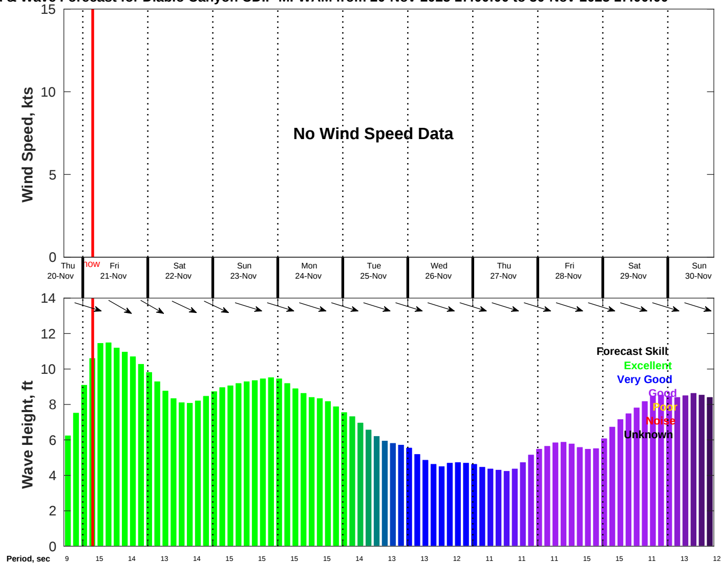
Wind & Wave Forecast for Diablo Canyon CDIP MFWAM from 20-Nov-2025 17:00:00 to 30-Nov-2025 17:00:00
