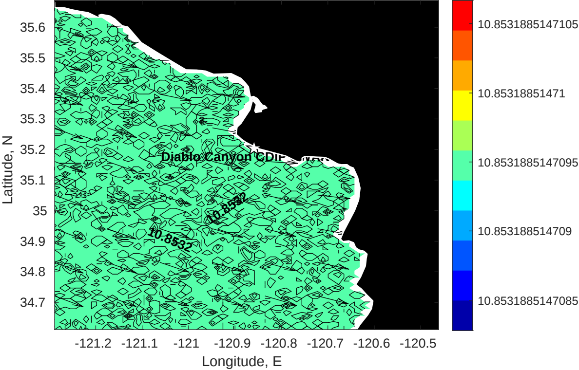
Wave Period (sec) for Diablo Canyon CDIP SWAN at 19-Nov-2025 18:00:00
